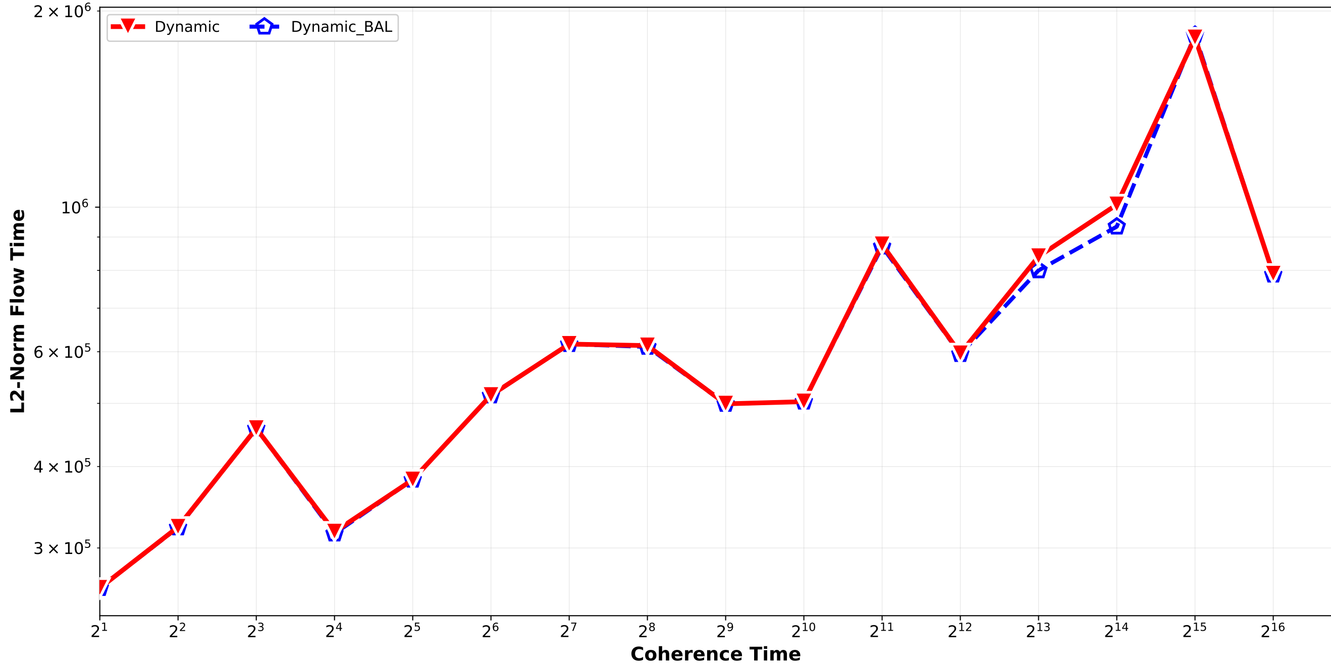
Dynamic vs Dynamic_BAL - L2 Norm Flow Time Bounded_Pareto_combination_random H64_H512_H4096 / triplet_1
