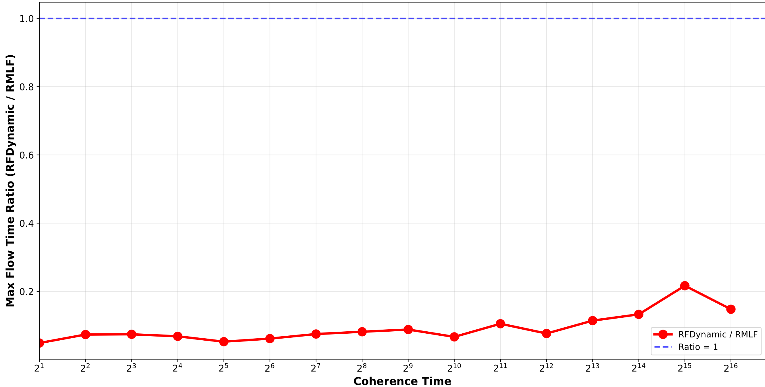
RFDynamic vs RMLF - Max Flow Time Ratio Bounded_Pareto_combination_random H64_H512_H4096 / triplet_1
