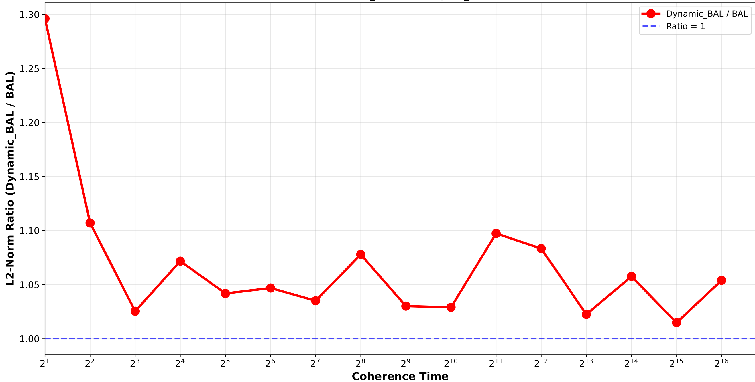
Dynamic_BAL vs BAL - L2 Norm Ratio Bounded_Pareto_combination_random H32768_H262144 / pair_4
