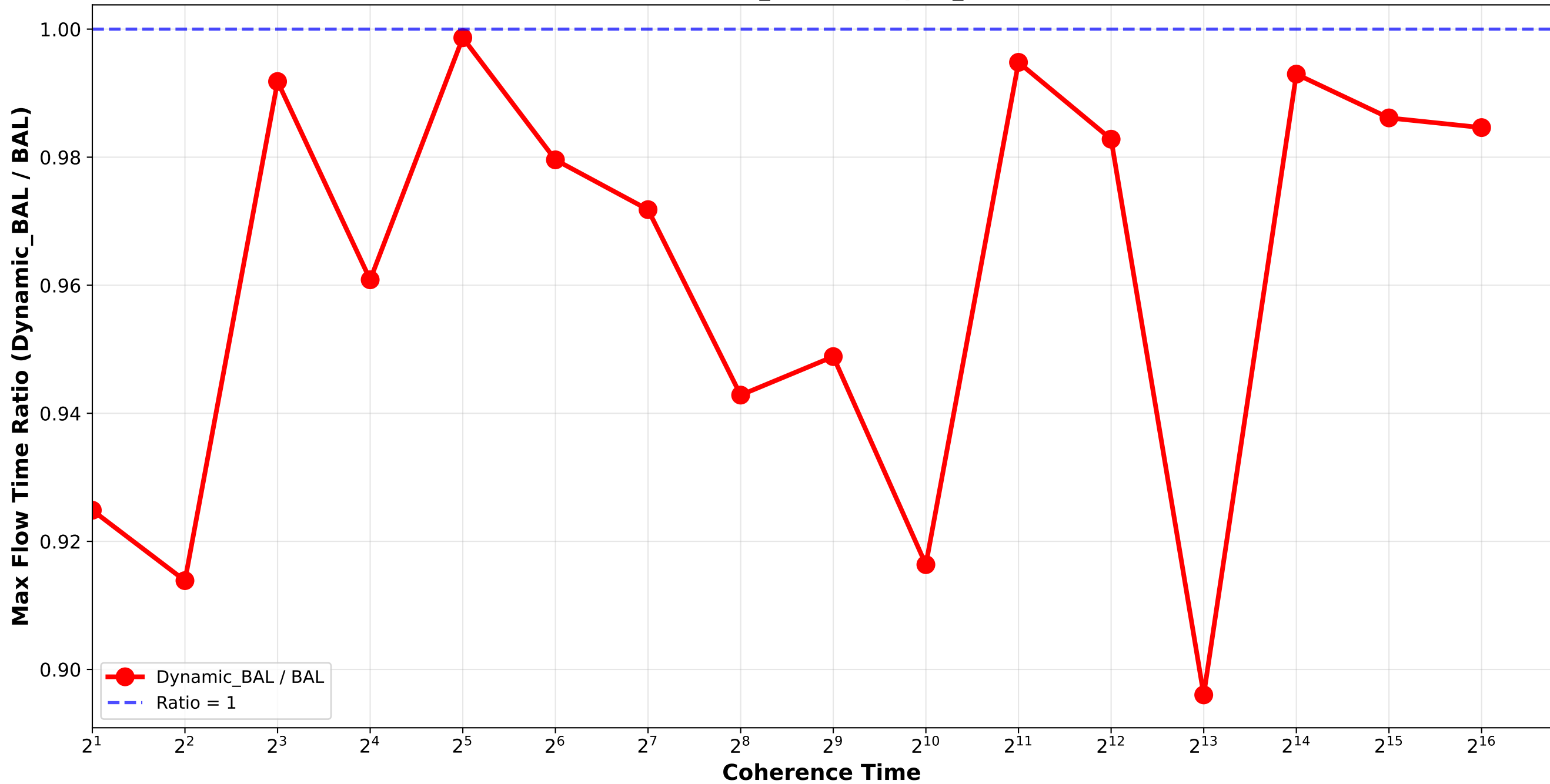
Dynamic_BAL vs BAL - Max Flow Time Ratio Bounded_Pareto_combination_random H32768_H262144 / pair_4
