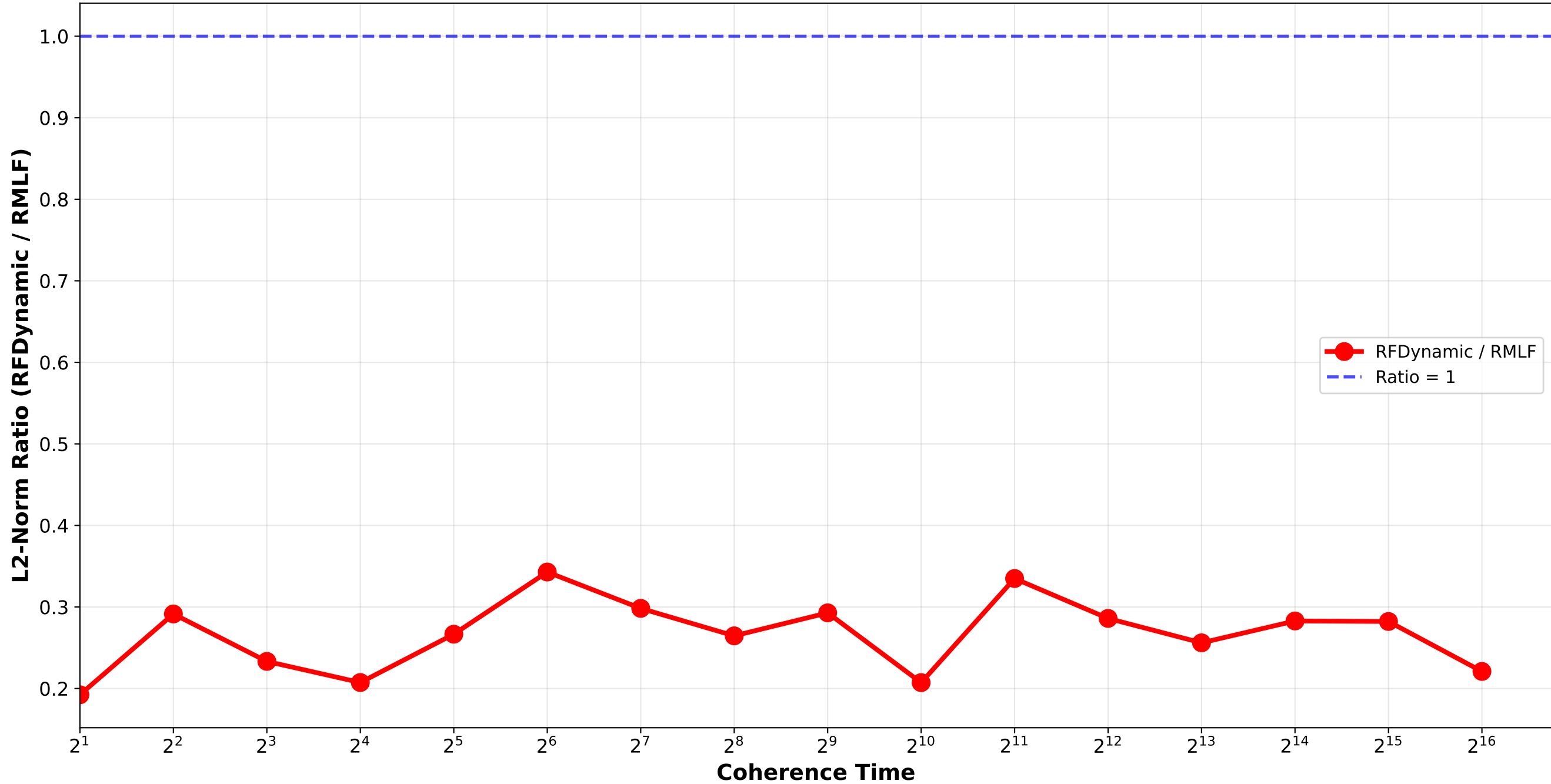
RFDynamic vs RMLF - L2 Norm Ratio Bounded_Pareto_combination_random H32768_H262144 / pair_4
