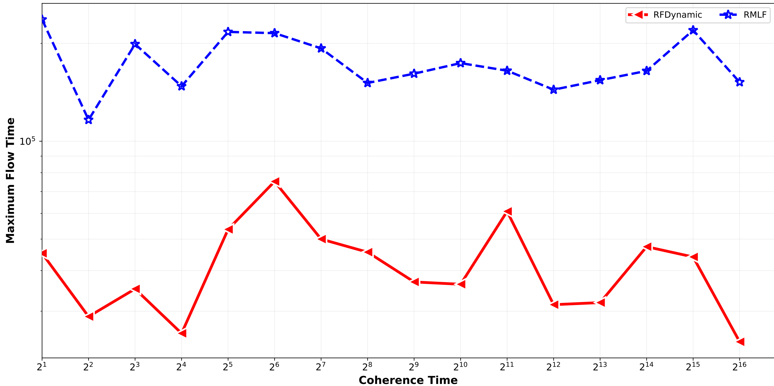
RFDynamic vs RMLF - Maximum Flow Time Bounded_Pareto_combination_random H32768_H262144 / pair_4
