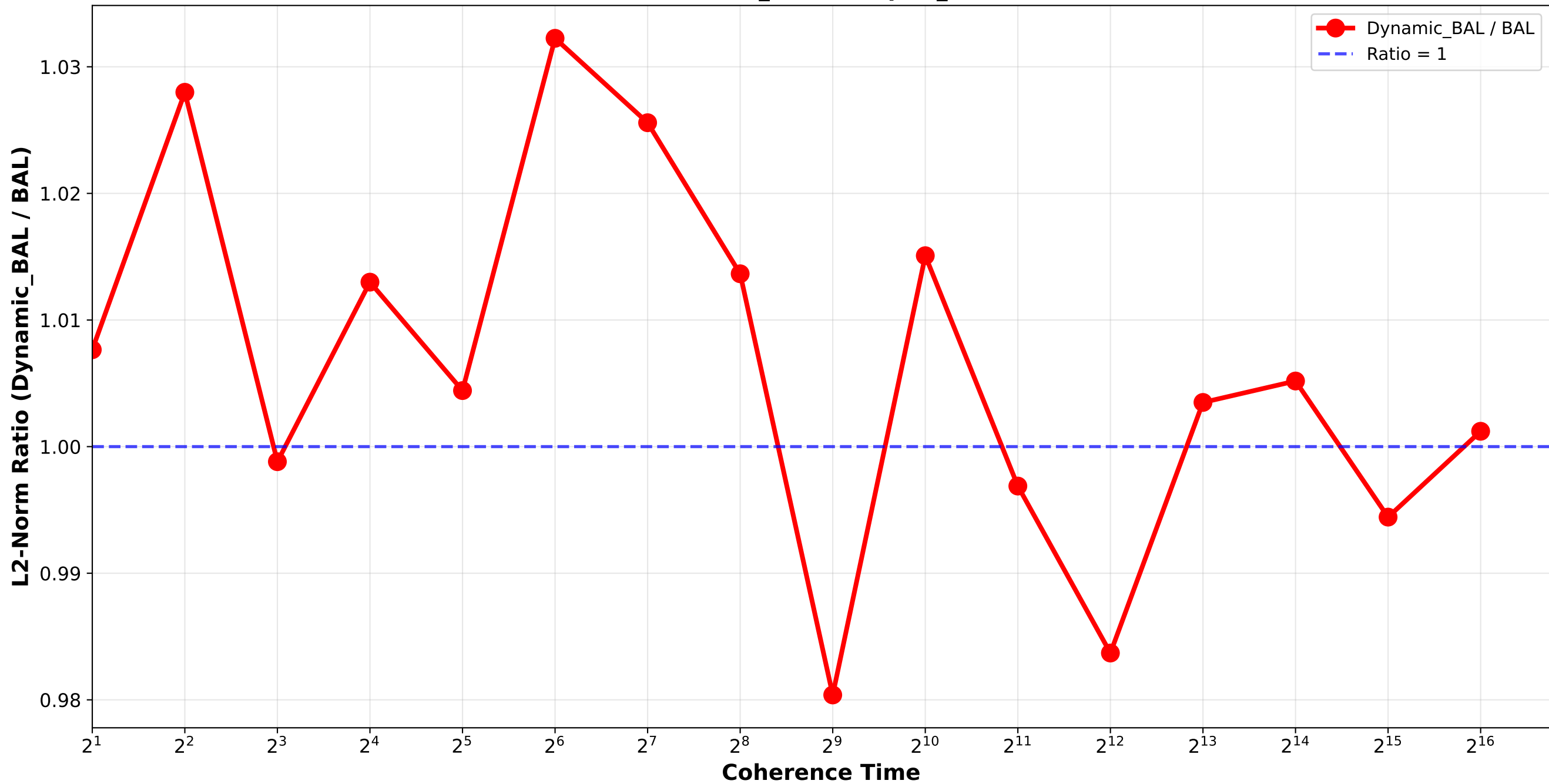
Dynamic_BAL vs BAL - L2 Norm Ratio Bounded_Pareto_combination_random H4096_H32768 / pair_3
