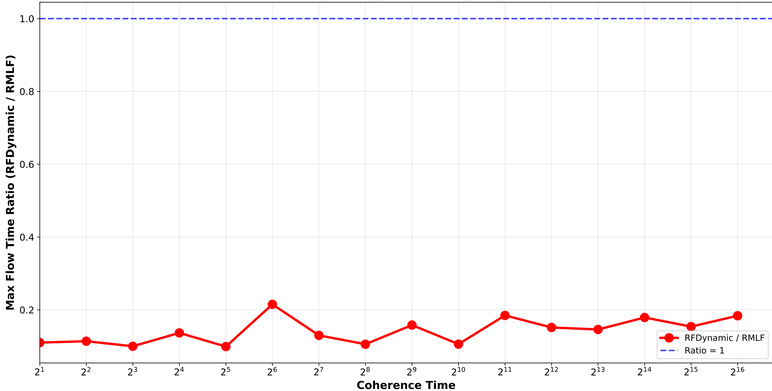
RFDynamic vs RMLF - Max Flow Time Ratio Bounded_Pareto_combination_random H4096_H32768 / pair_3
