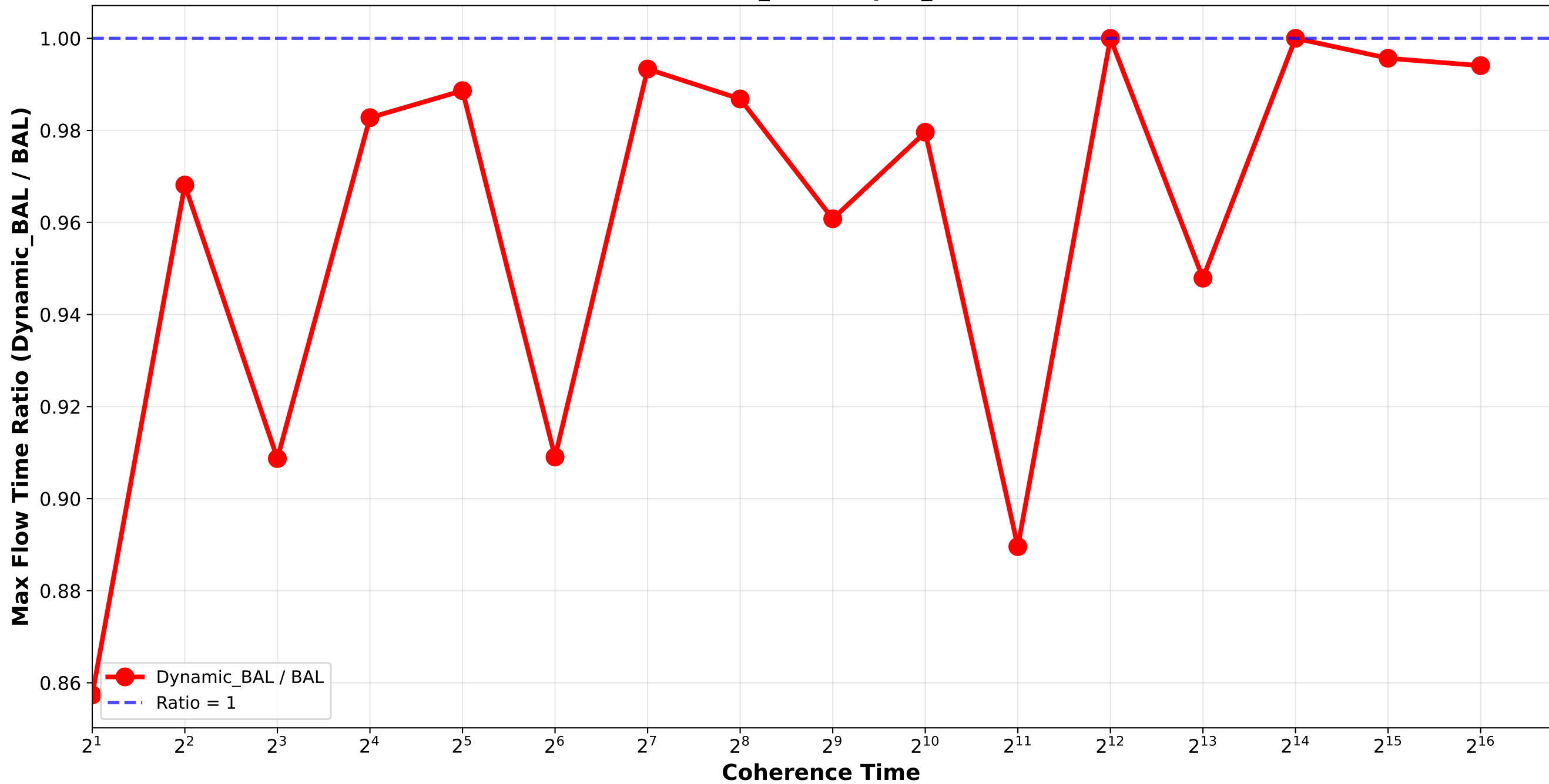
Dynamic_BAL vs BAL - Max Flow Time Ratio Bounded_Pareto_combination_random H512_H4096 / pair_2
