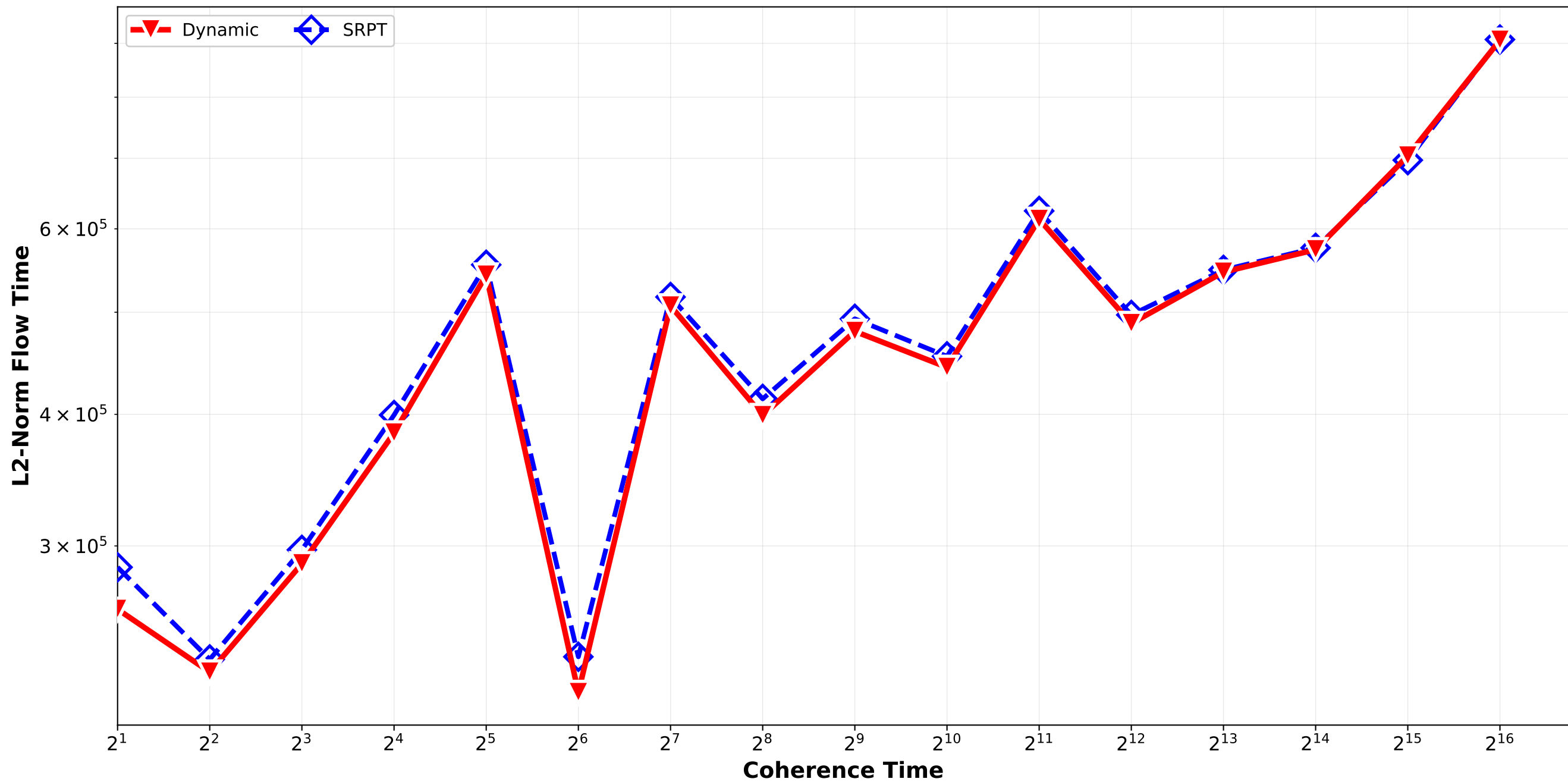
Dynamic vs SRPT - L2 Norm Flow Time Bounded_Pareto_combination_random H512_H4096 / pair_2
