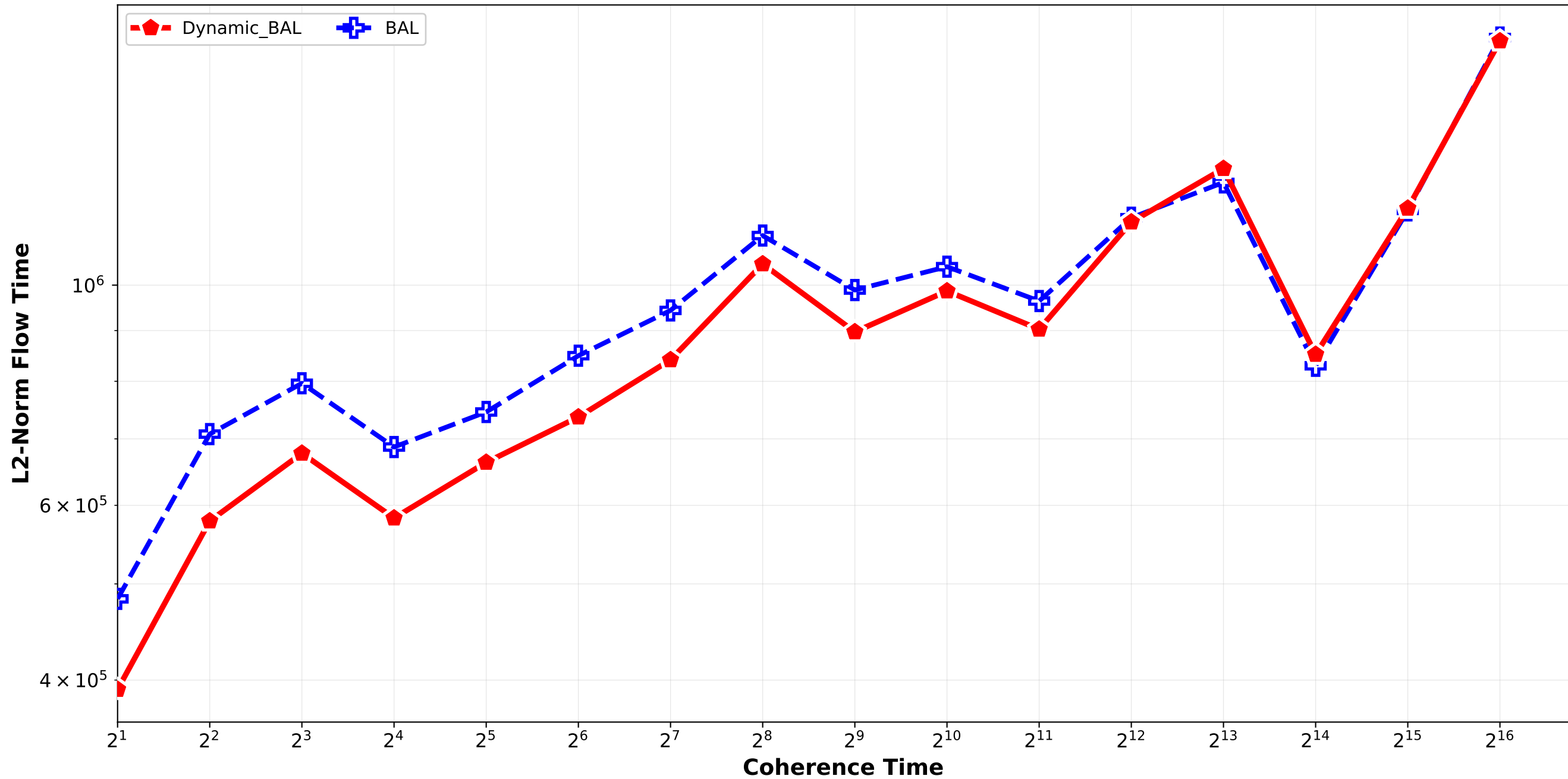
Dynamic_BAL vs BAL - L2 Norm Flow Time Bounded_Pareto_combination_random H64_H512 / pair_1
