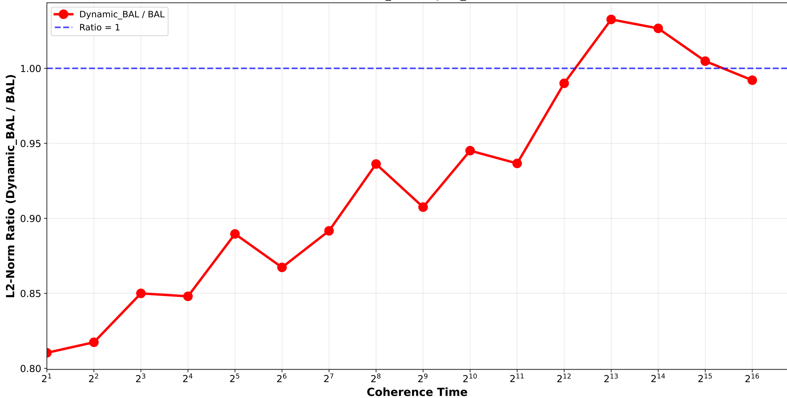
Dynamic_BAL vs BAL - L2 Norm Ratio Bounded_Pareto_combination_random H64_H512 / pair_1
