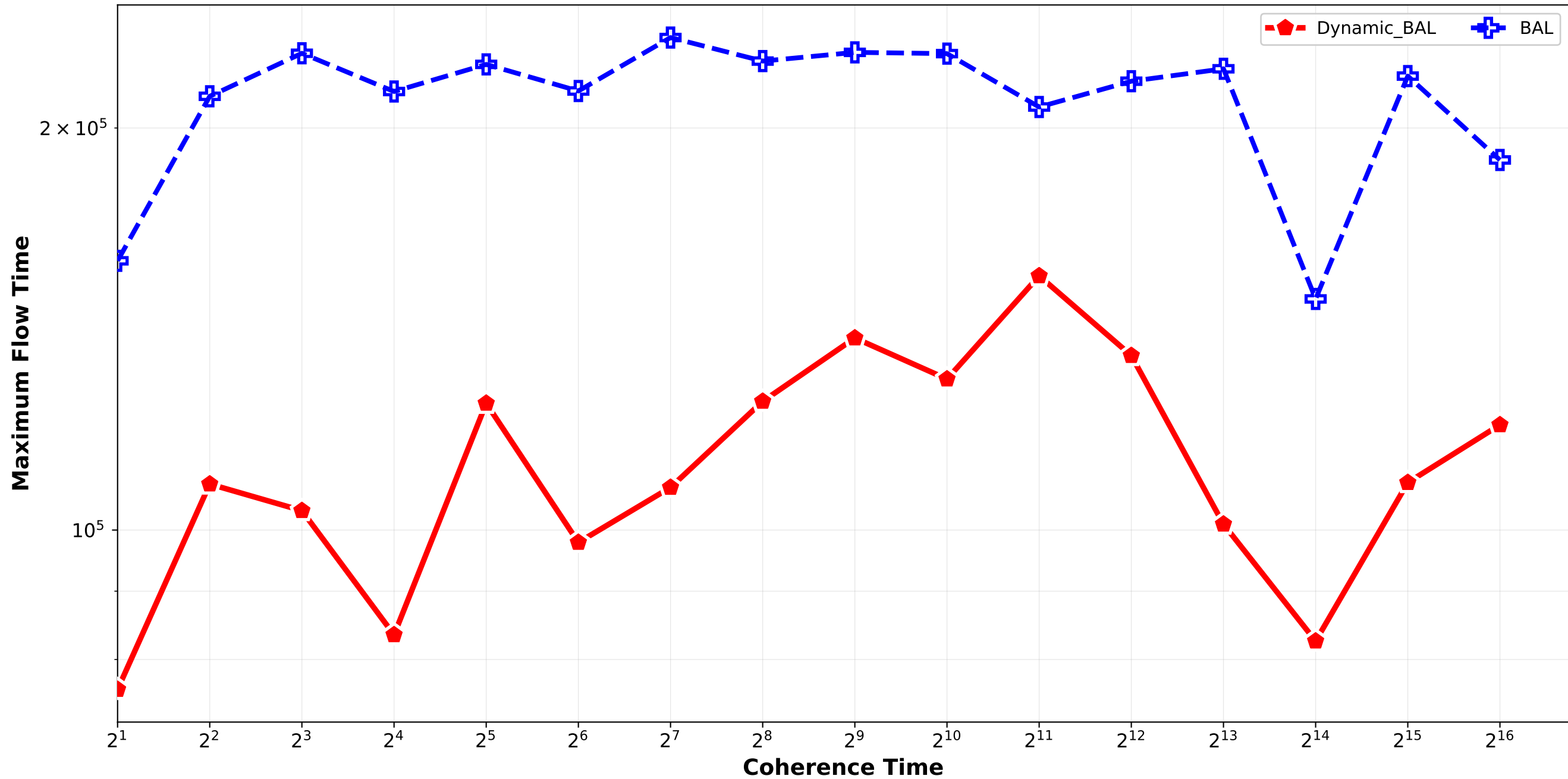
Dynamic_BAL vs BAL - Maximum Flow Time Bounded_Pareto_combination_random H64_H512 / pair_1
