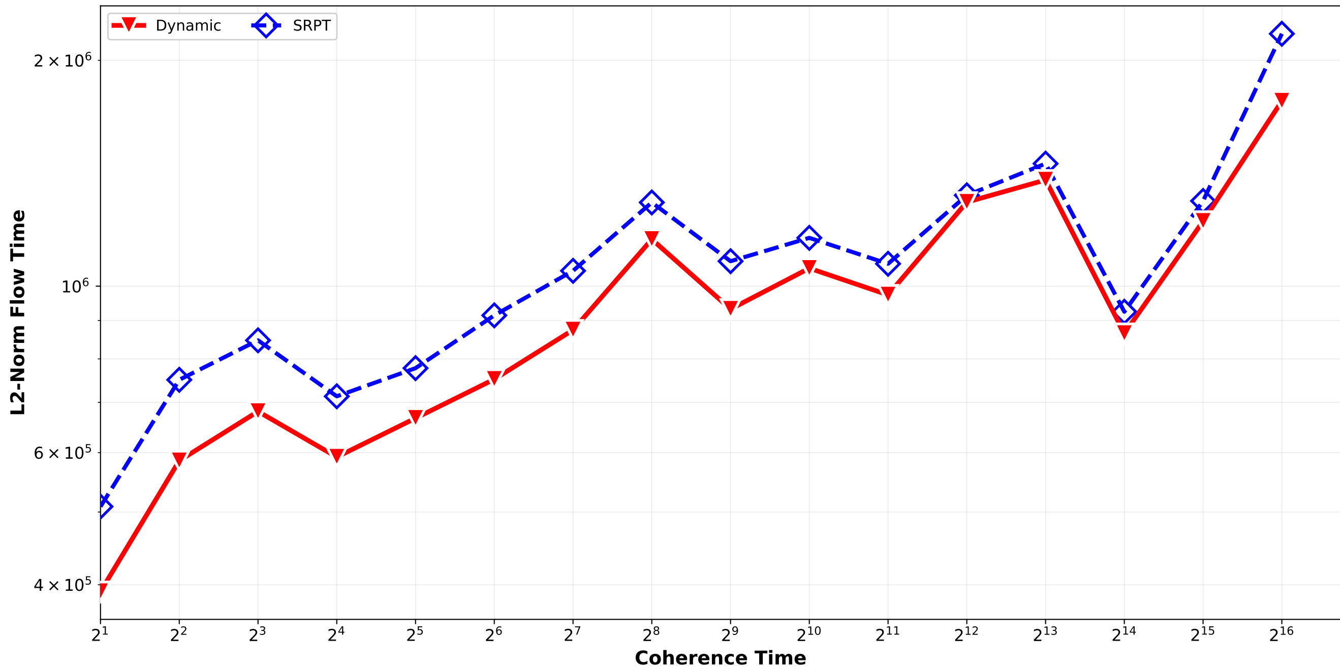
Dynamic vs SRPT - L2 Norm Flow Time Bounded_Pareto_combination_random H64_H512 / pair_1
