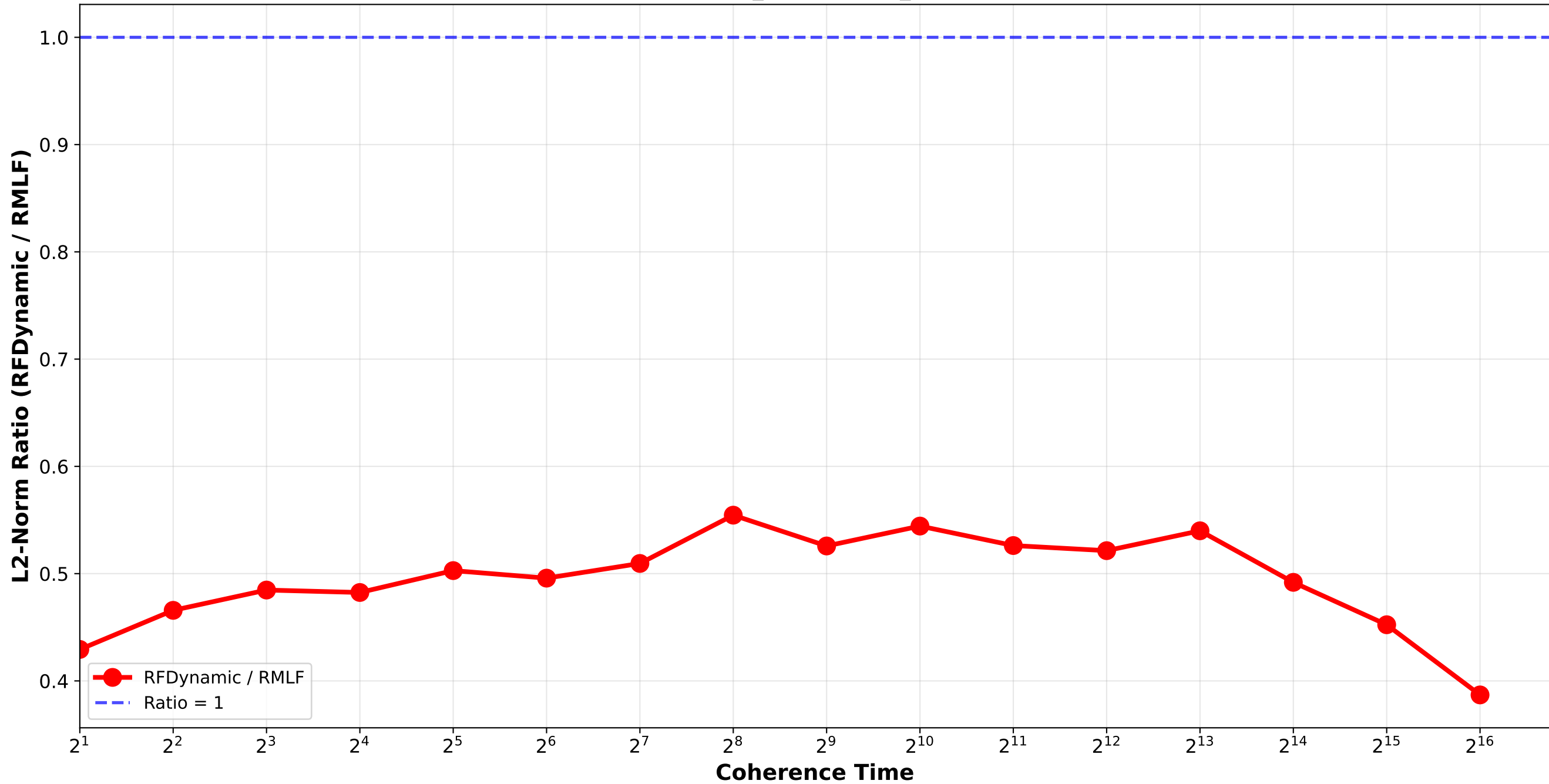
RFDynamic vs RMLF - L2 Norm Ratio Bounded_Pareto_combination_random H64_H512 / pair_1
