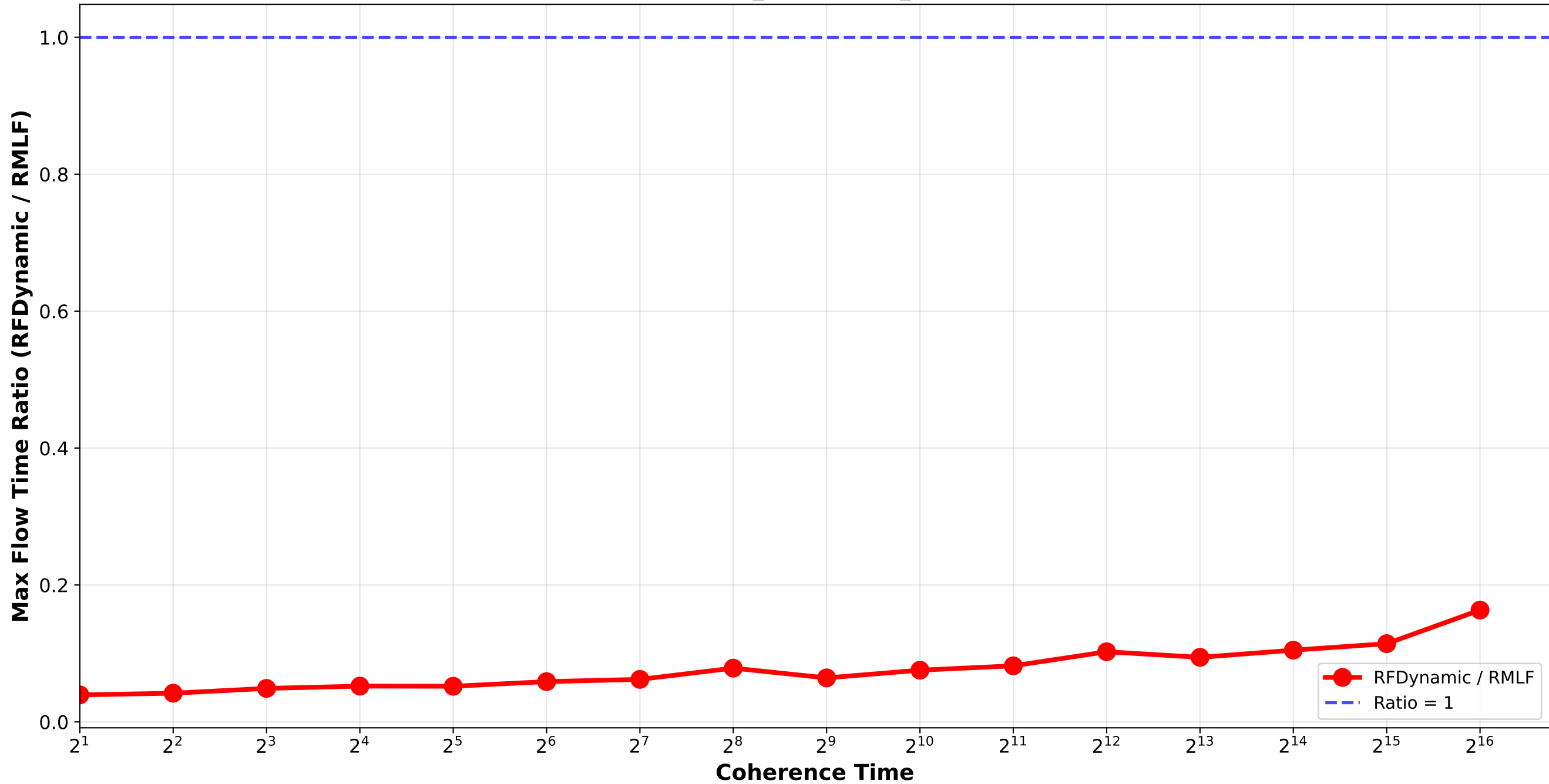
RFDynamic vs RMLF - Max Flow Time Ratio Bounded_Pareto_combination_random H64_H512 / pair_1
