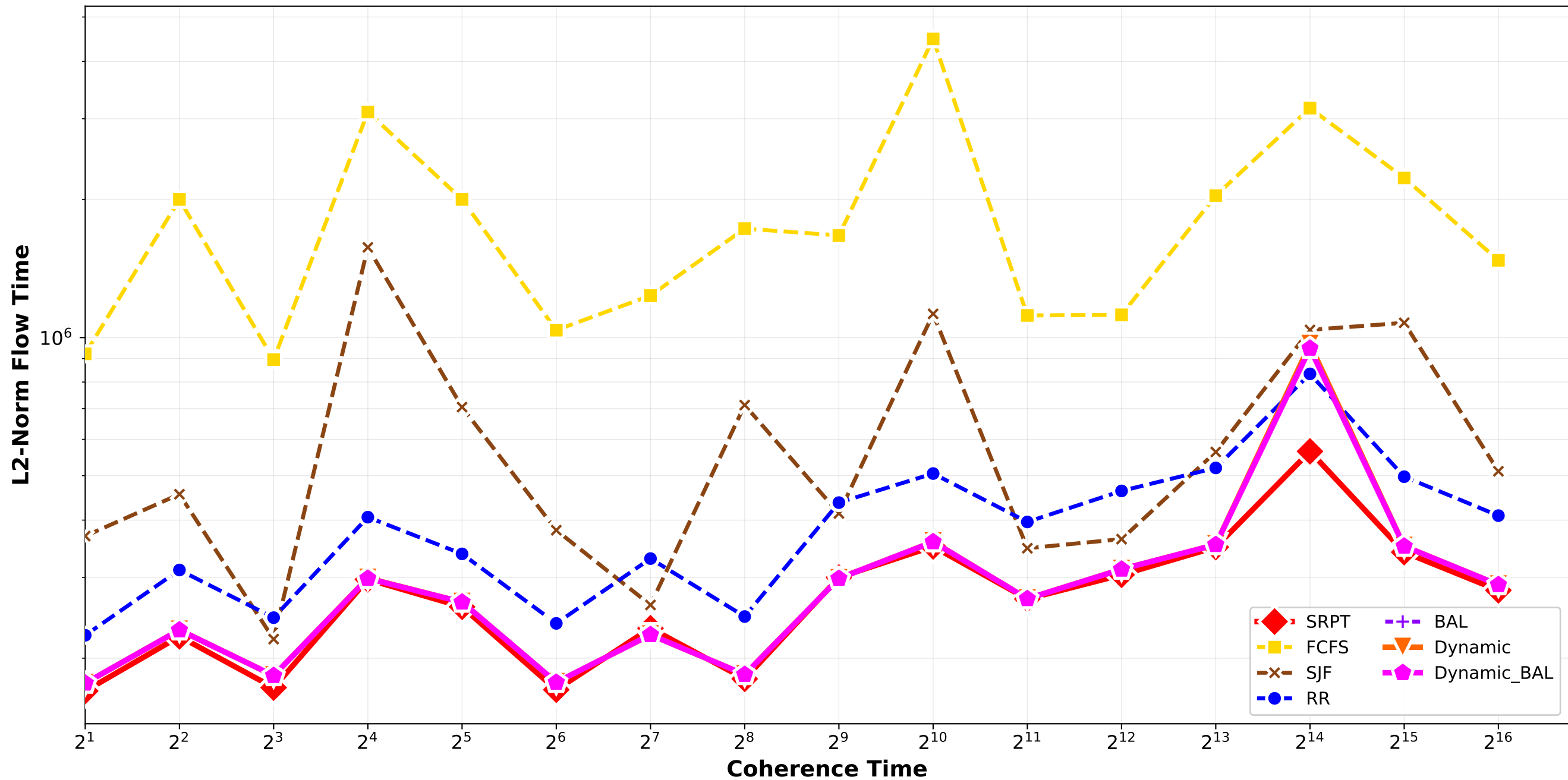
Clairvoyant Algorithms - L2 Norm Flow Time Bounded_Pareto_combination_softrandom H512_H4096_H32768_H262144 / quadruplet_2
