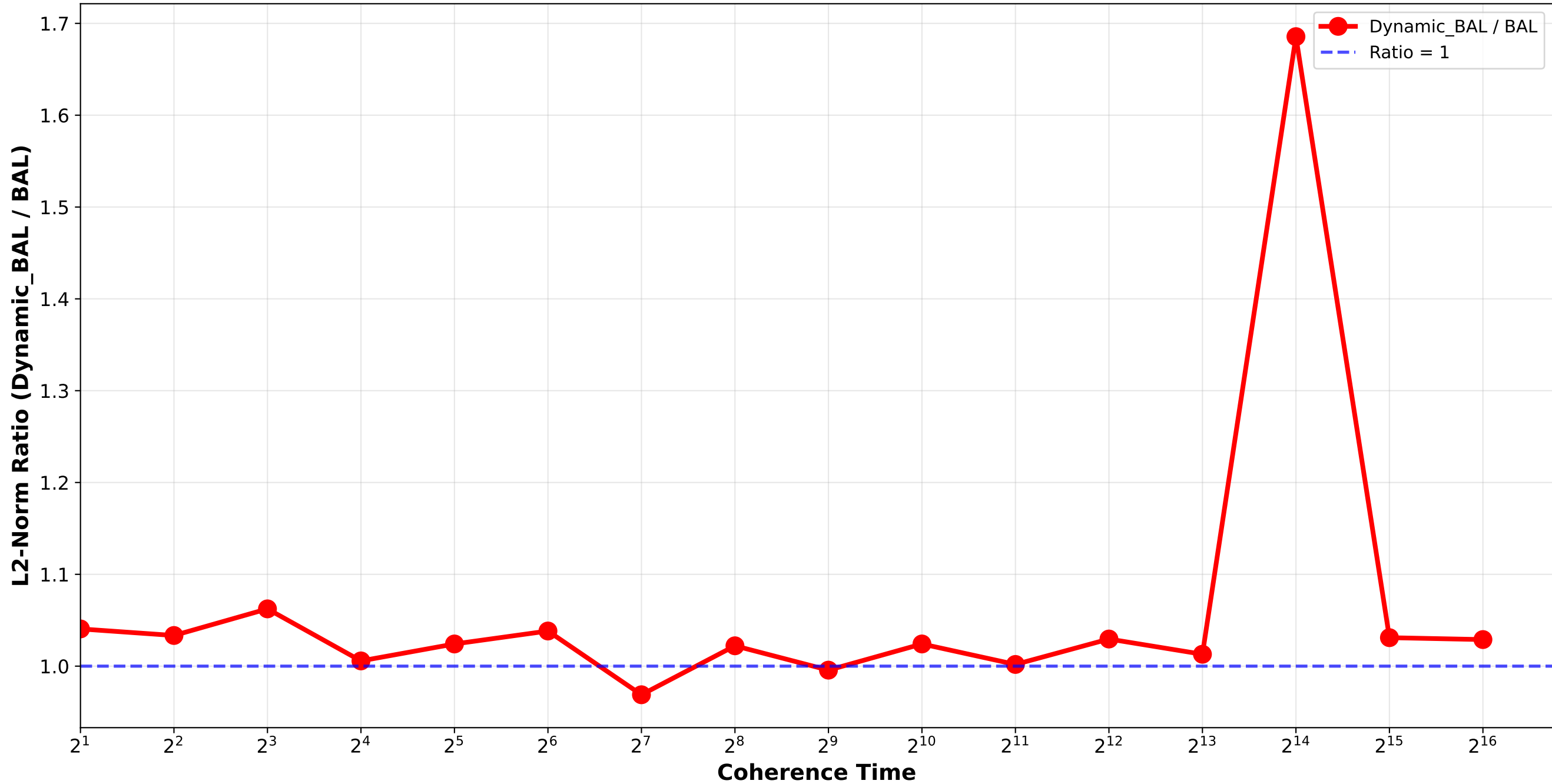
Dynamic_BAL vs BAL - L2 Norm Ratio Bounded_Pareto_combination_softrandom H512_H4096_H32768_H262144 / quadruplet_2
