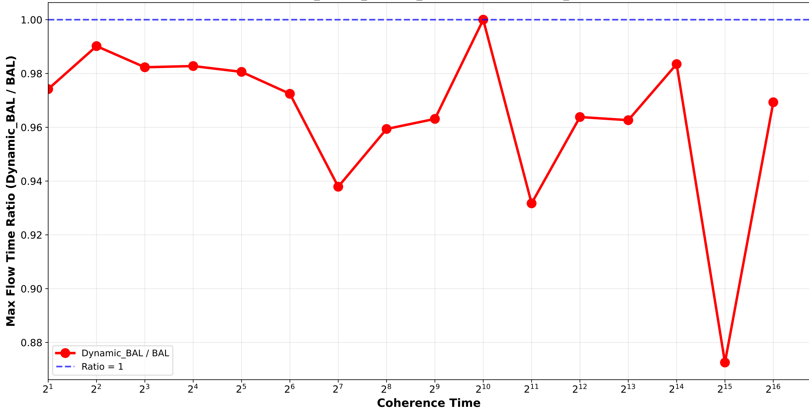
Dynamic_BAL vs BAL - Max Flow Time Ratio Bounded_Pareto_combination_softrandom H512_H4096_H32768_H262144 / quadruplet_2
