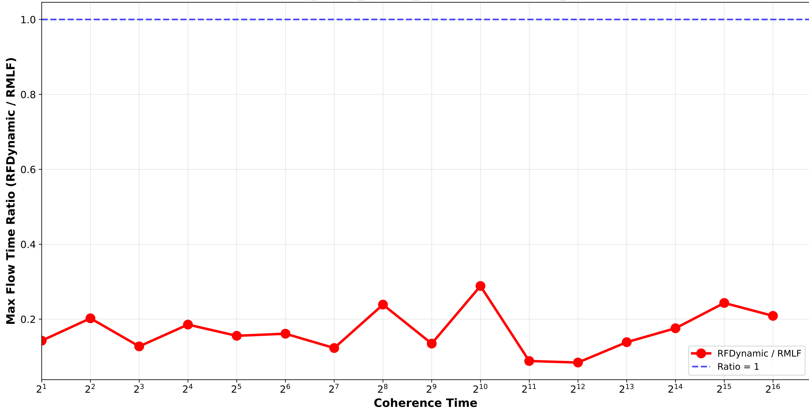
RFDynamic vs RMLF - Max Flow Time Ratio Bounded_Pareto_combination_softrandom H512_H4096_H32768_H262144 / quadruplet_2
