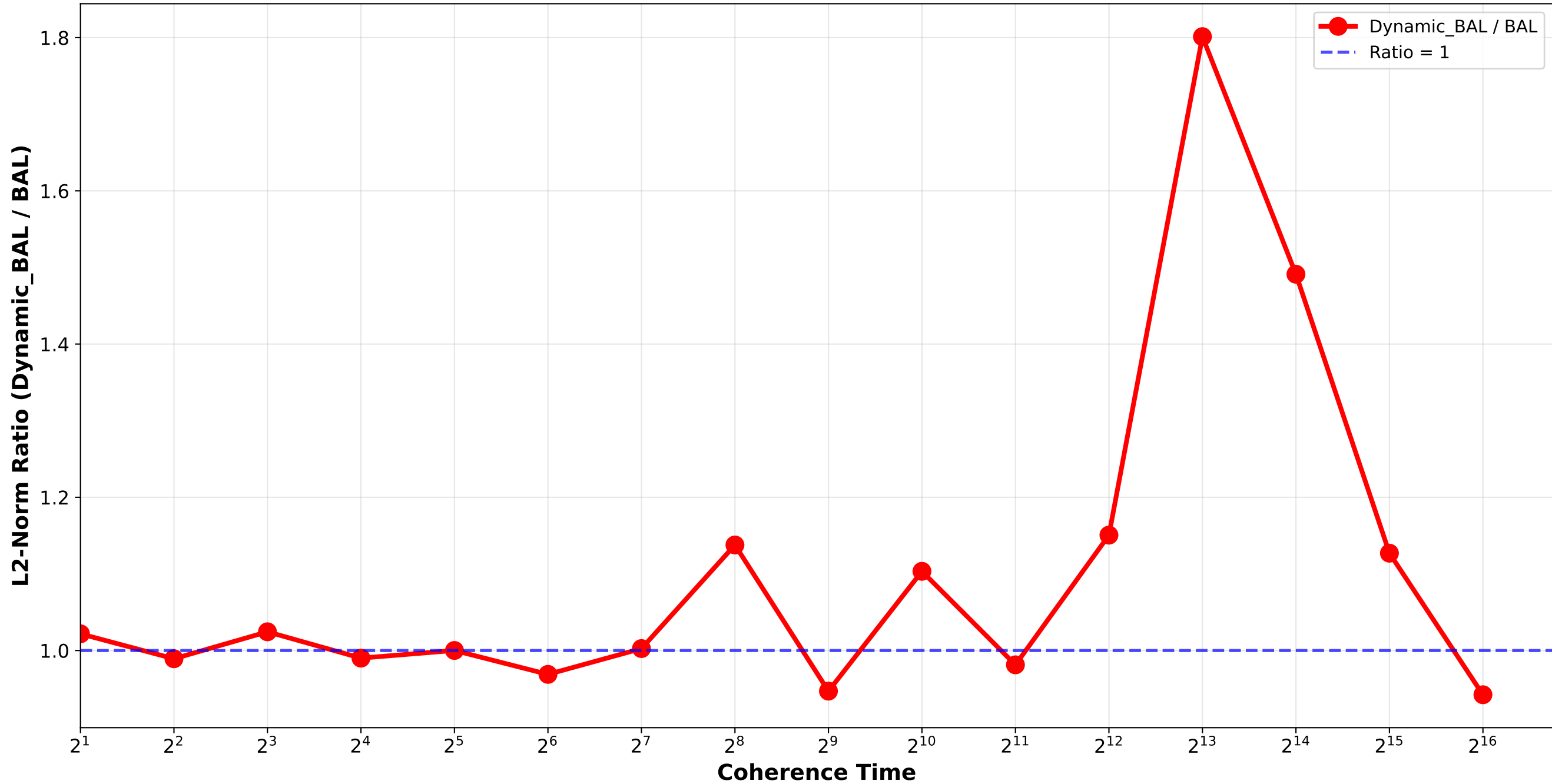
Dynamic_BAL vs BAL - L2 Norm Ratio Bounded_Pareto_combination_softrandom H64_H512_H4096_H32768 / quadruplet_1
