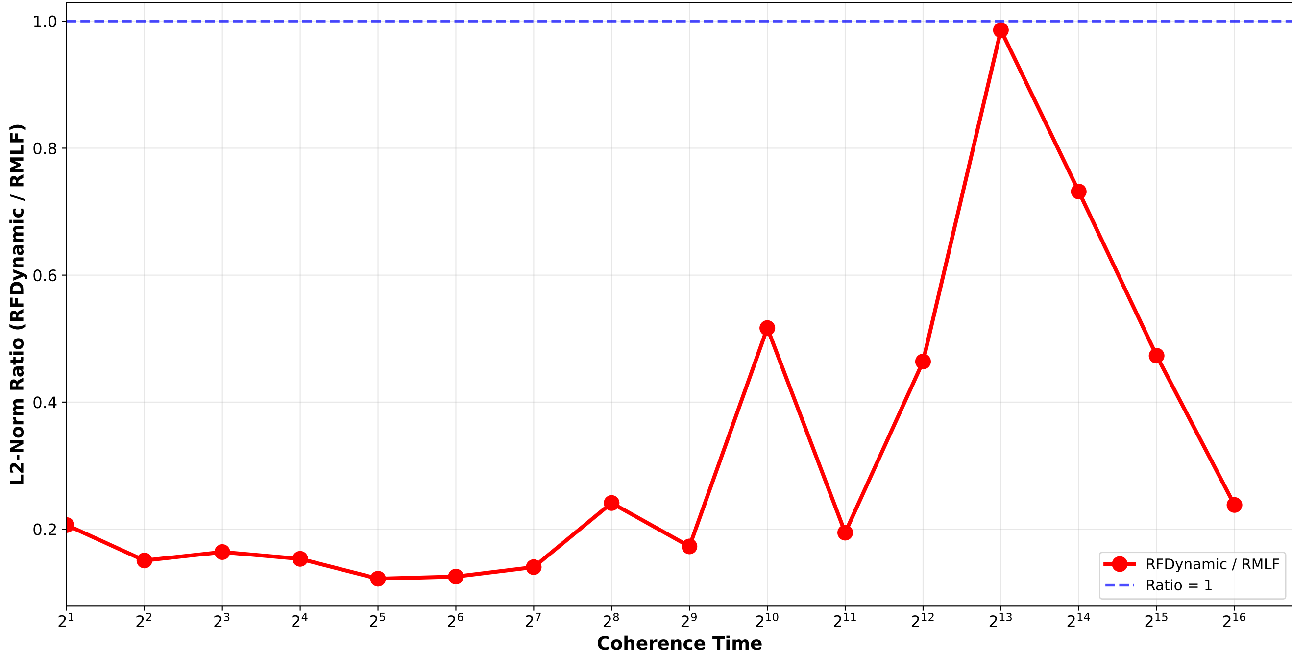
RFDynamic vs RMLF - L2 Norm Ratio Bounded_Pareto_combination_softrandom H64_H512_H4096_H32768 / quadruplet_1
