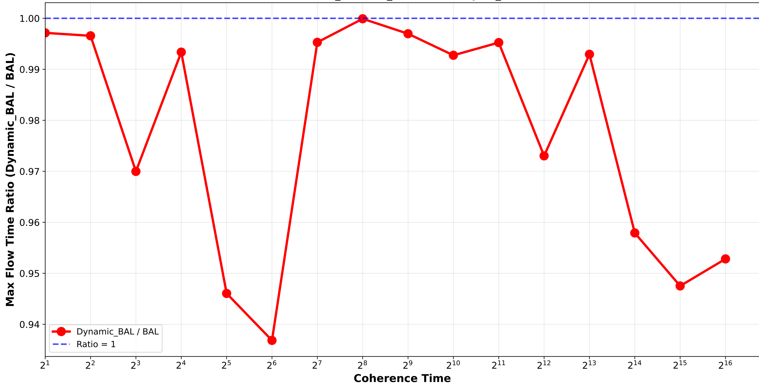
Dynamic_BAL vs BAL - Max Flow Time Ratio Bounded_Pareto_combination_softrandom H4096_H32768_H262144 / triplet_3
