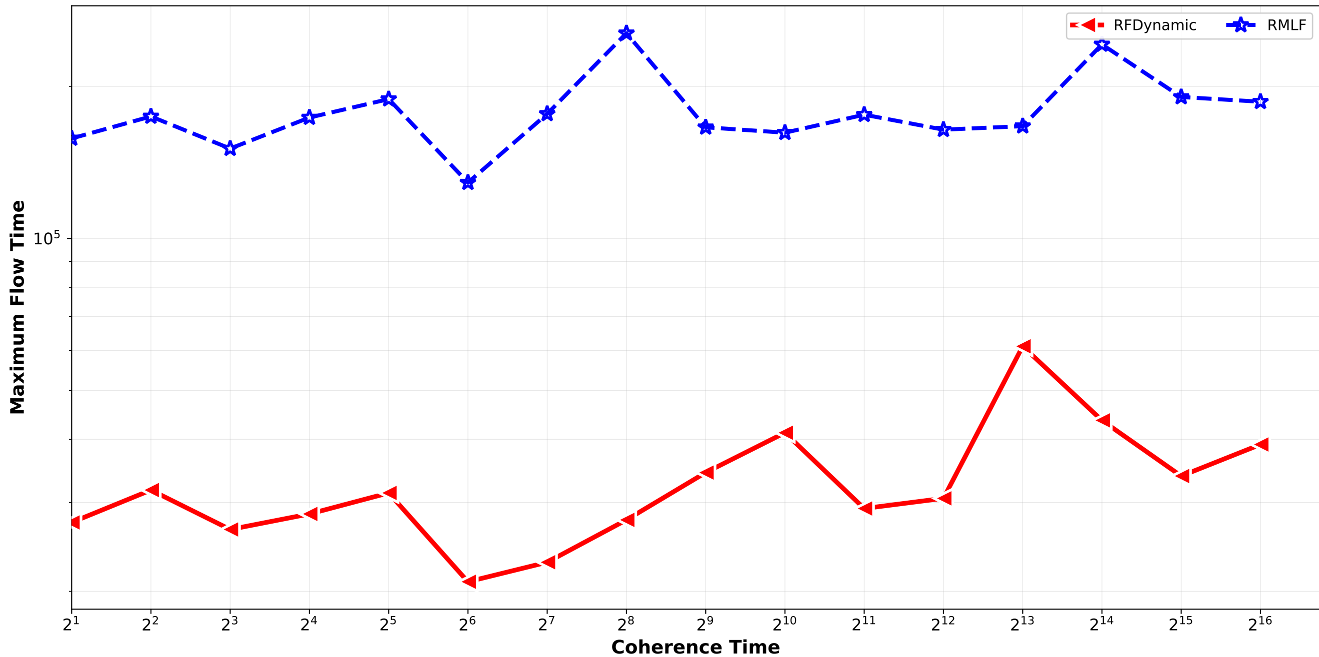
RFDynamic vs RMLF - Maximum Flow Time Bounded_Pareto_combination_softrandom H4096_H32768_H262144 / triplet_3
