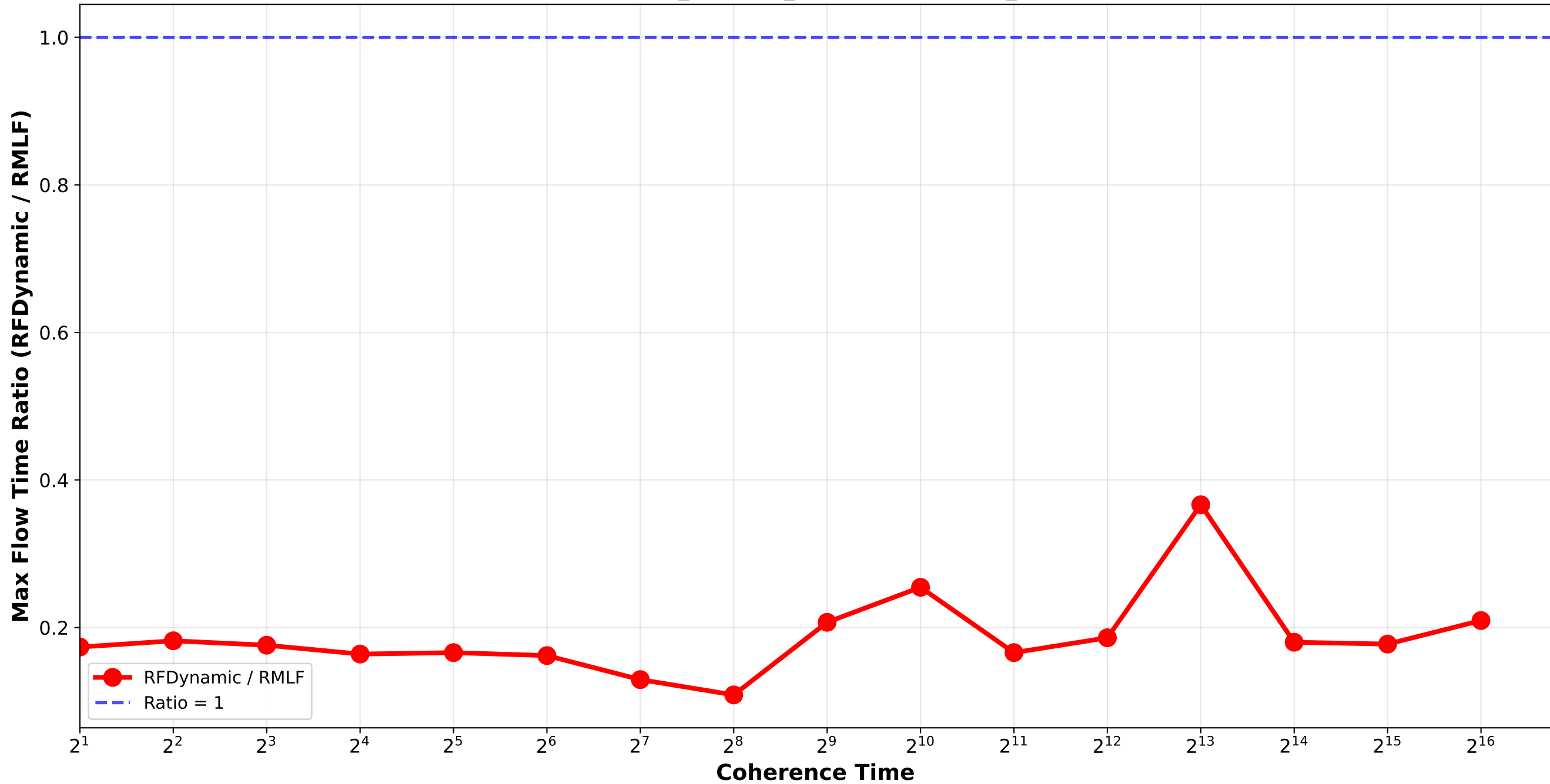
RFDynamic vs RMLF - Max Flow Time Ratio Bounded_Pareto_combination_softrandom H4096_H32768_H262144 / triplet_3
