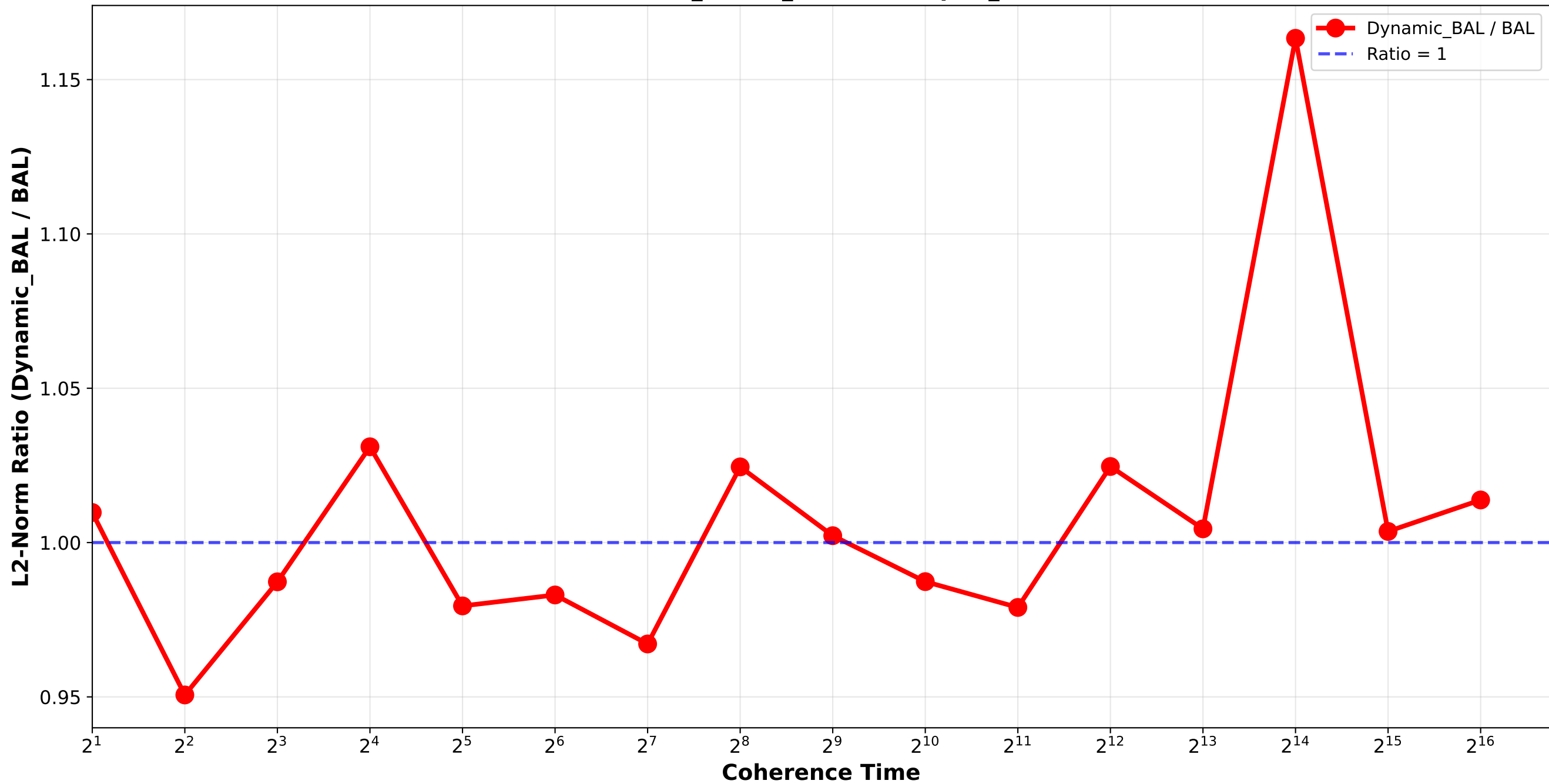
Dynamic_BAL vs BAL - L2 Norm Ratio Bounded_Pareto_combination_softrandom H512_H4096_H32768 / triplet_2
