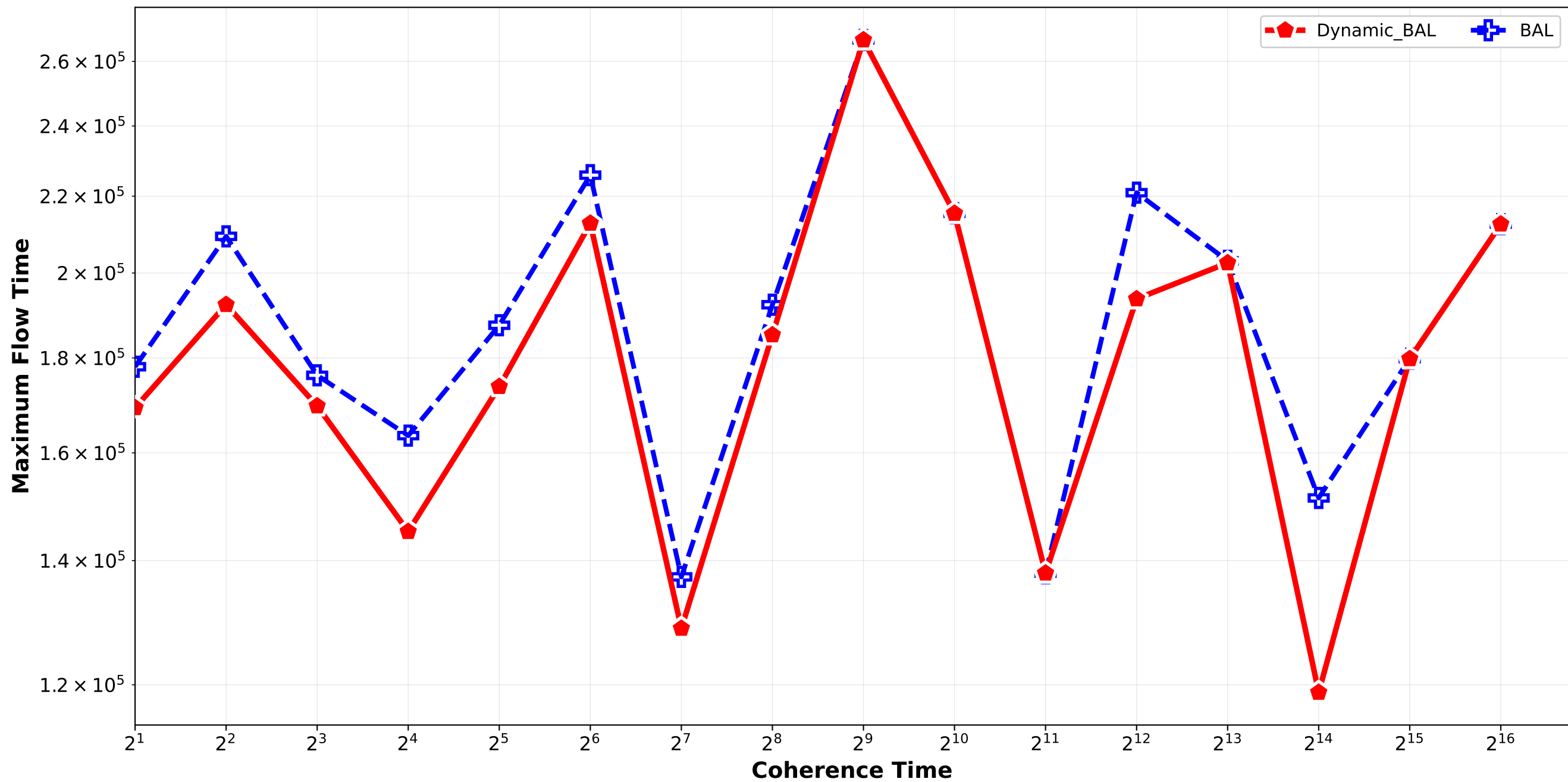
Dynamic_BAL vs BAL - Maximum Flow Time Bounded_Pareto_combination_softrandom H512_H4096_H32768 / triplet_2
