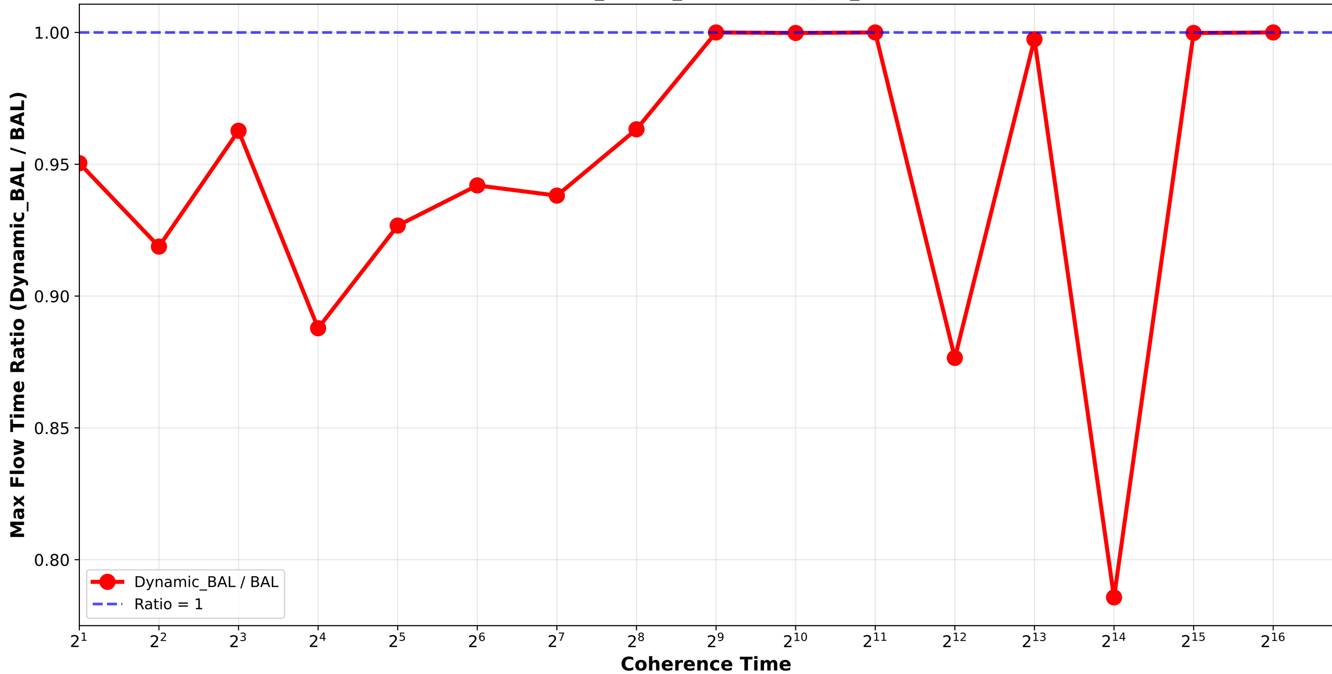
Dynamic_BAL vs BAL - Max Flow Time Ratio Bounded_Pareto_combination_softrandom H512_H4096_H32768 / triplet_2
