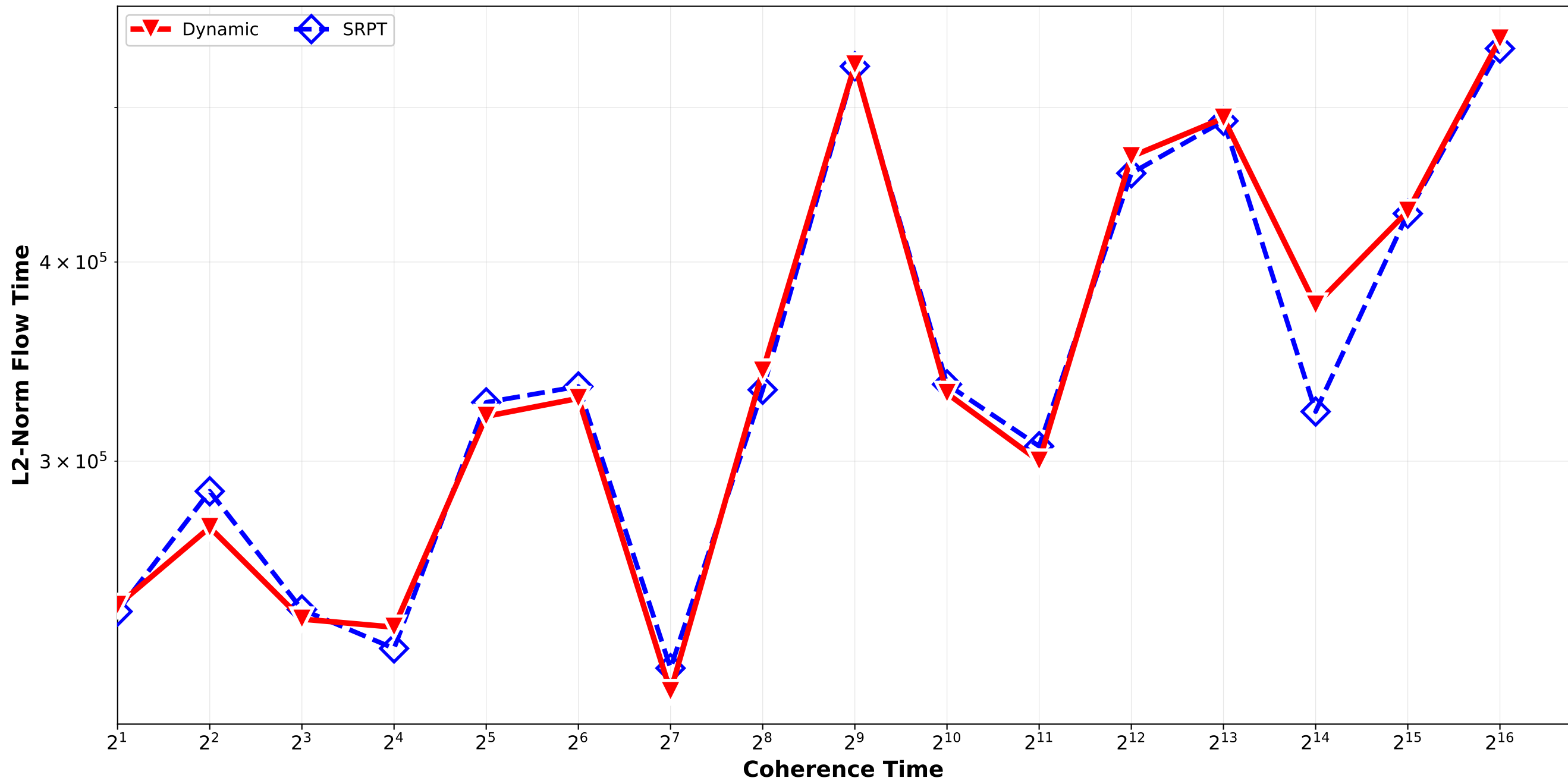
Dynamic vs SRPT - L2 Norm Flow Time Bounded_Pareto_combination_softrandom H512_H4096_H32768 / triplet_2
