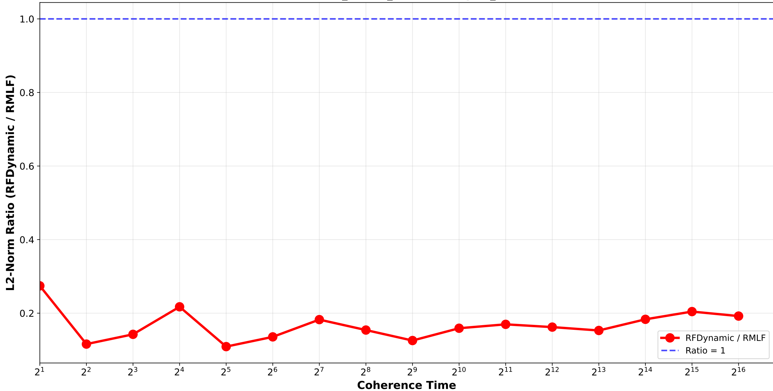
RFDynamic vs RMLF - L2 Norm Ratio Bounded_Pareto_combination_softrandom H512_H4096_H32768 / triplet_2
