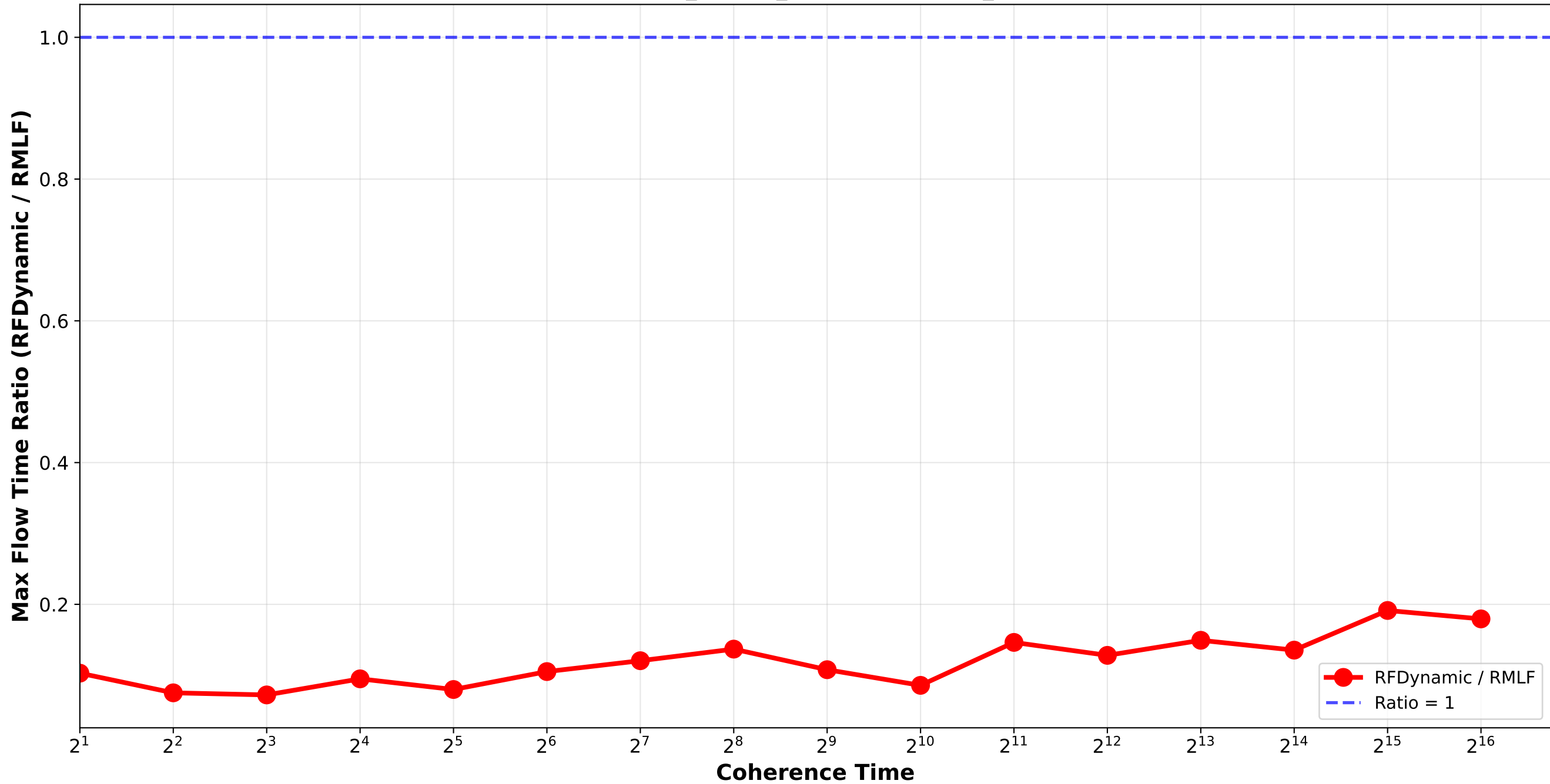
RFDynamic vs RMLF - Max Flow Time Ratio Bounded_Pareto_combination_softrandom H512_H4096_H32768 / triplet_2
