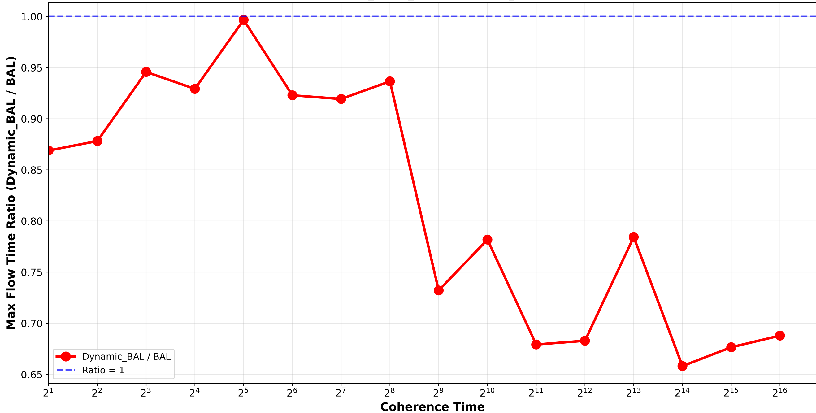
Dynamic_BAL vs BAL - Max Flow Time Ratio Bounded_Pareto_combination_softrandom H64_H512_H4096 / triplet_1
