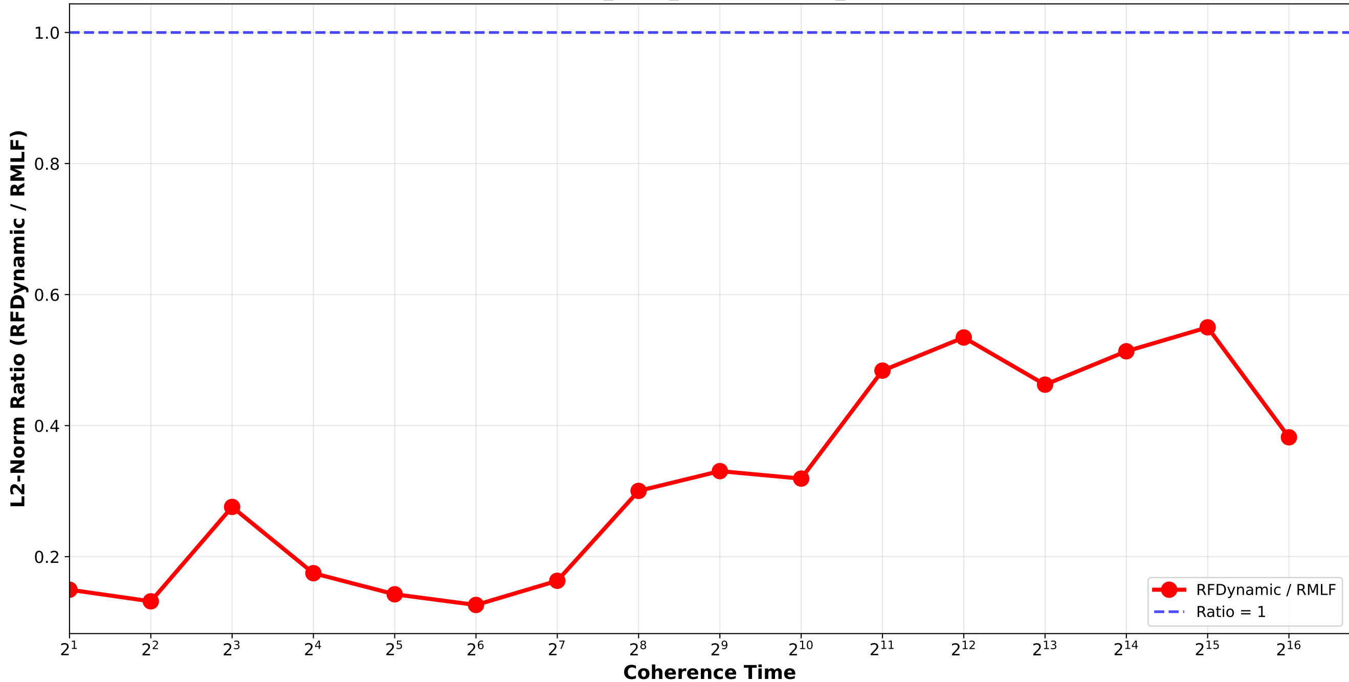
RFDynamic vs RMLF - L2 Norm Ratio Bounded_Pareto_combination_softrandom H64_H512_H4096 / triplet_1
