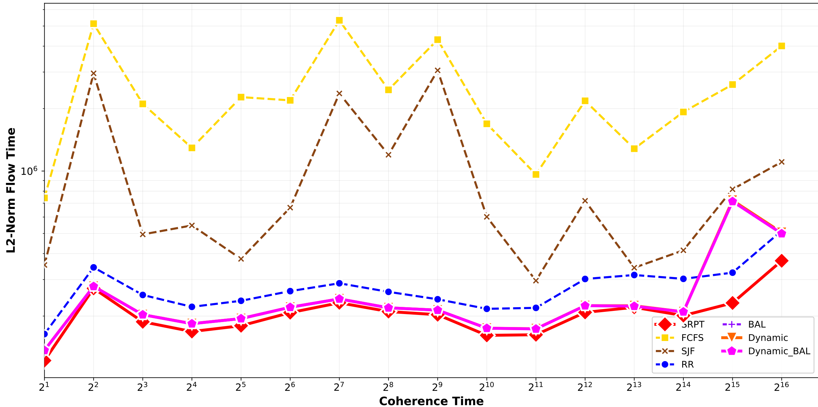
Clairvoyant Algorithms - L2 Norm Flow Time Bounded_Pareto_combination_softrandom H32768_H262144 / pair_4
