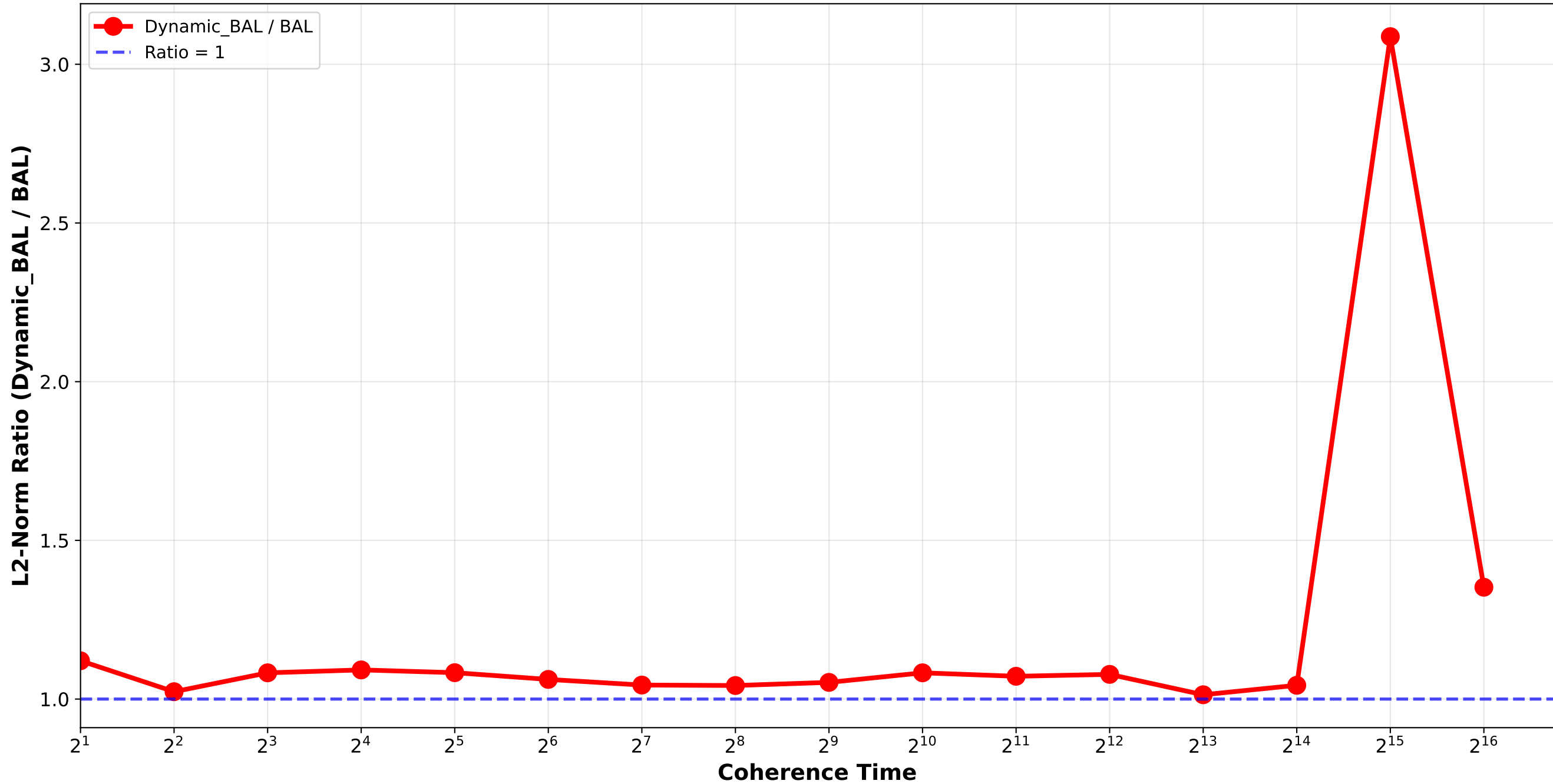
Dynamic_BAL vs BAL - L2 Norm Ratio Bounded_Pareto_combination_softrandom H32768_H262144 / pair_4
