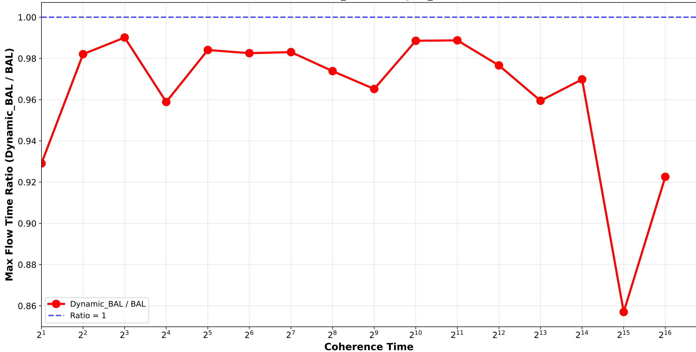
Dynamic_BAL vs BAL - Max Flow Time Ratio Bounded_Pareto_combination_softrandom H32768_H262144 / pair_4
