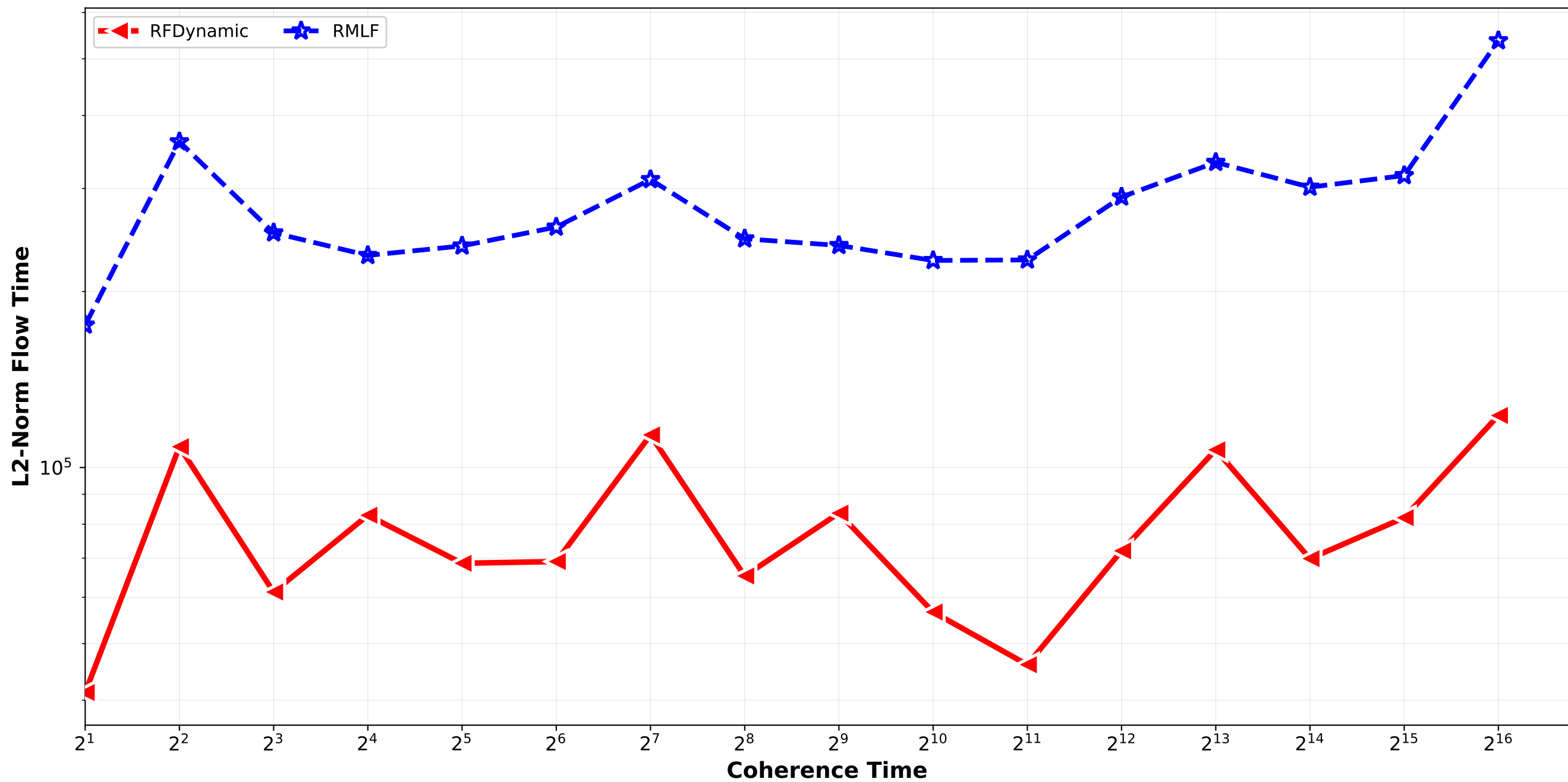
RFDynamic vs RMLF - L2 Norm Flow Time Bounded_Pareto_combination_softrandom H32768_H262144 / pair_4
