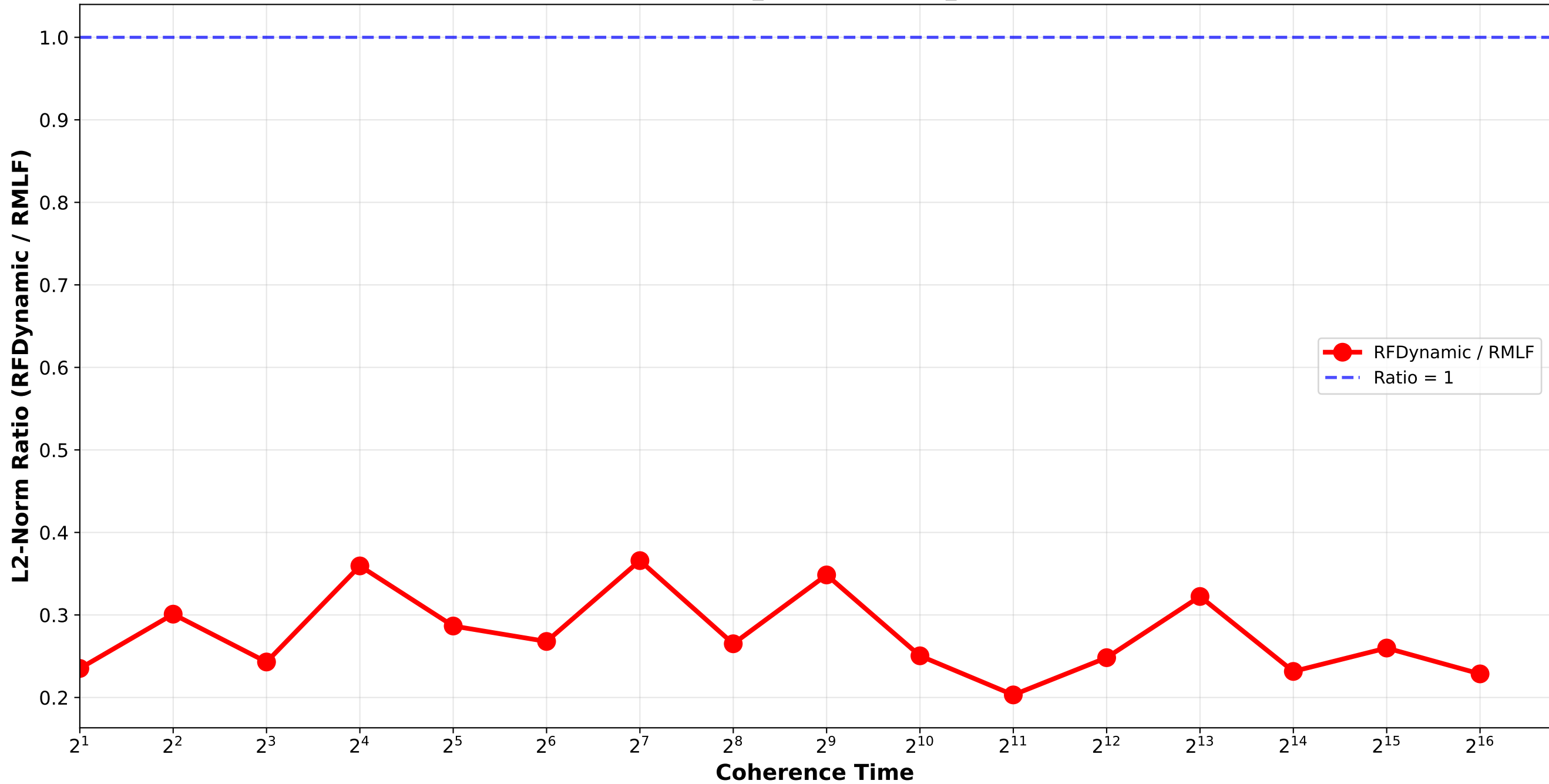
RFDynamic vs RMLF - L2 Norm Ratio Bounded_Pareto_combination_softrandom H32768_H262144 / pair_4
