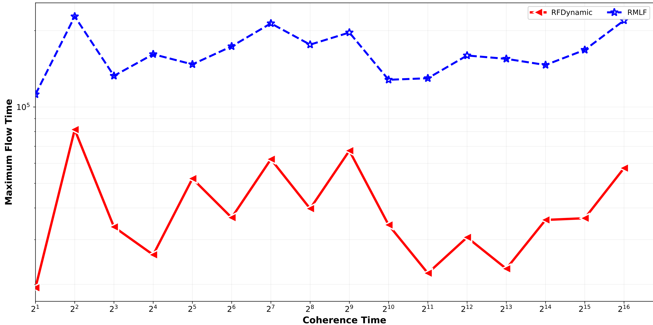
RFDynamic vs RMLF - Maximum Flow Time Bounded_Pareto_combination_softrandom H32768_H262144 / pair_4
