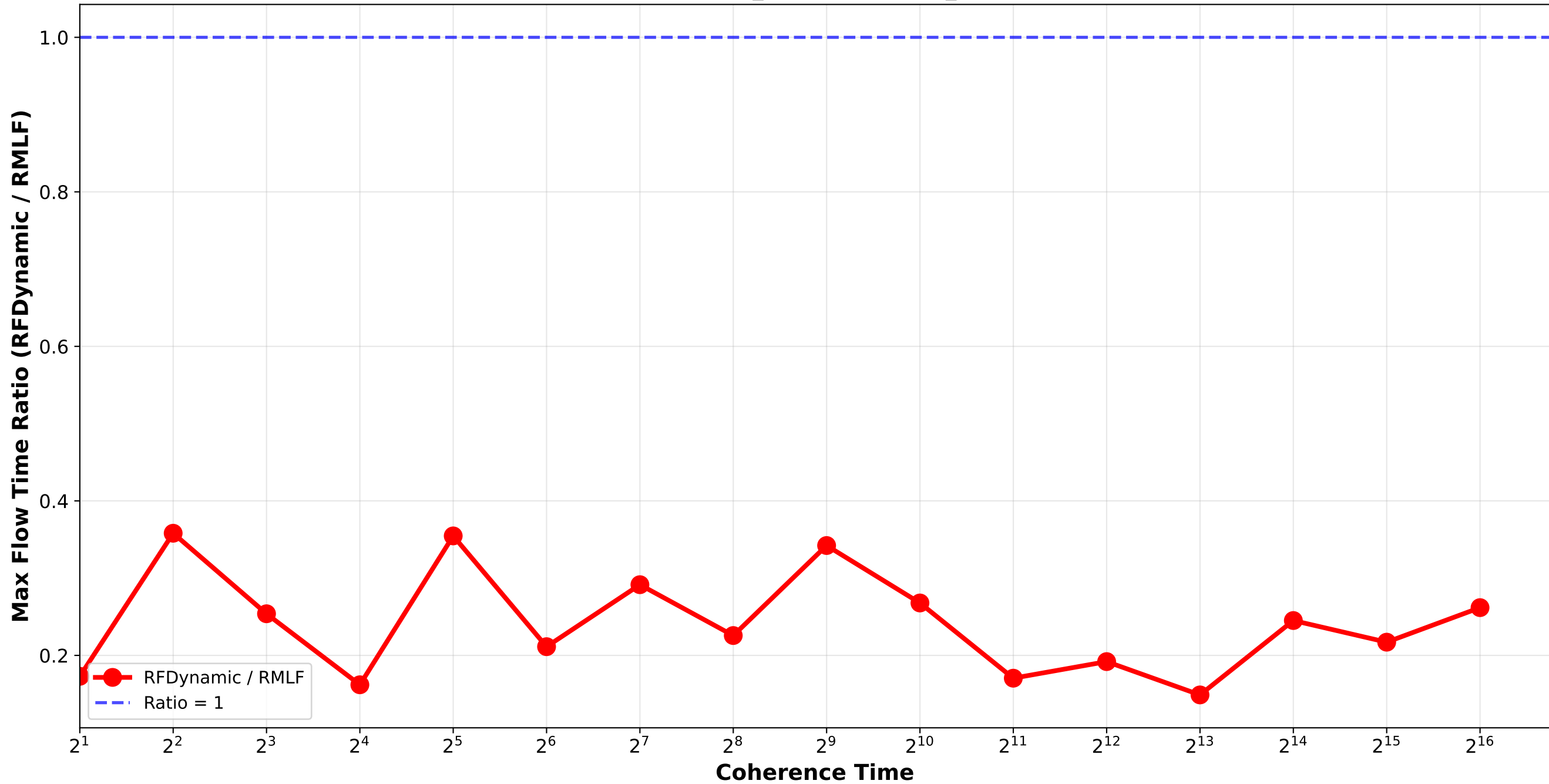
RFDynamic vs RMLF - Max Flow Time Ratio Bounded_Pareto_combination_softrandom H32768_H262144 / pair_4
