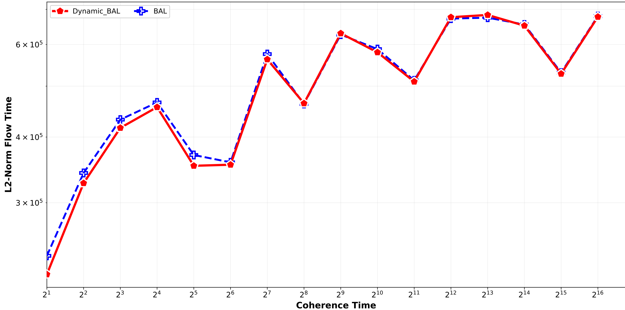
Dynamic_BAL vs BAL - L2 Norm Flow Time Bounded_Pareto_combination_softrandom H512_H4096 / pair_2
