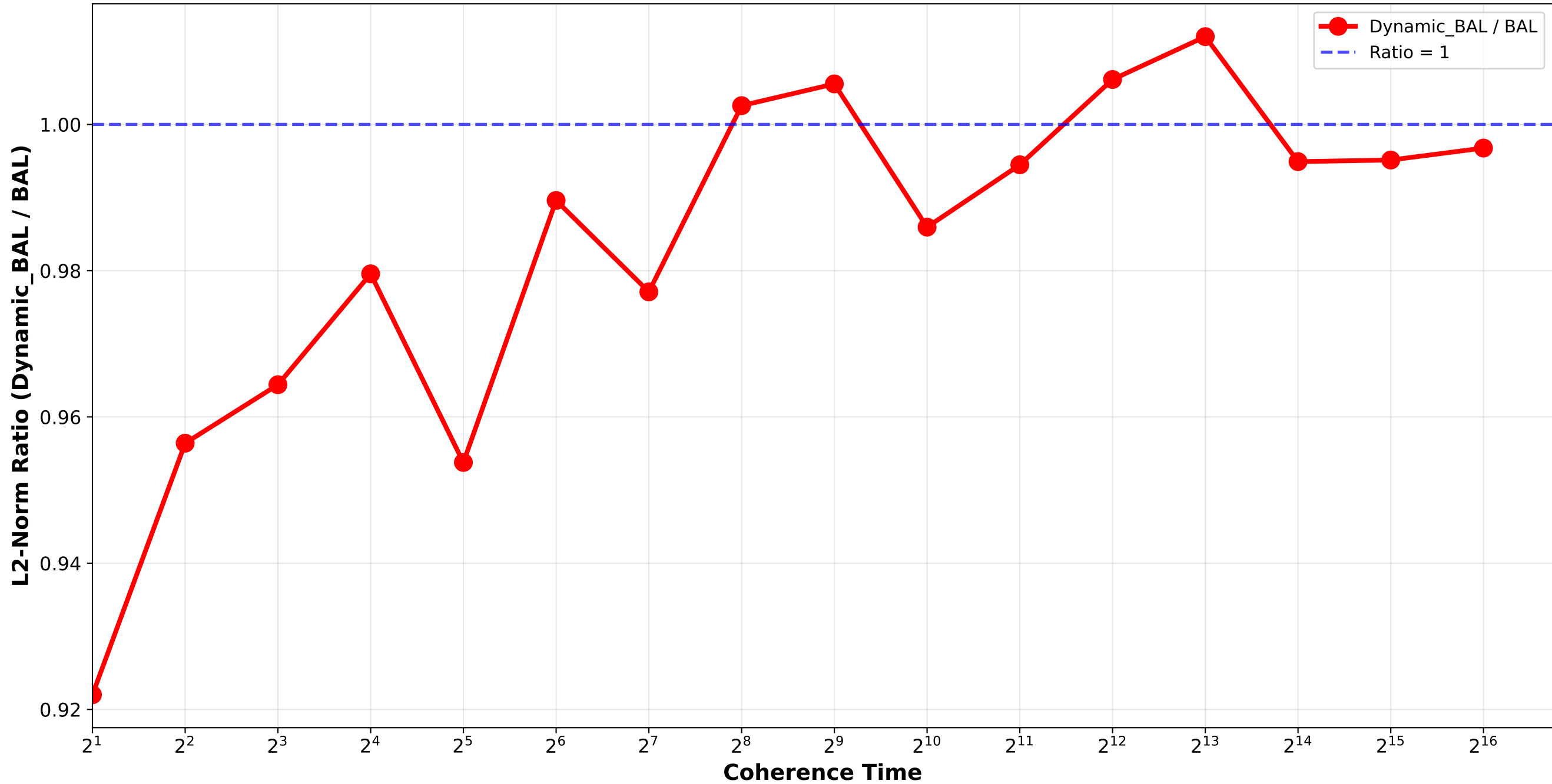
Dynamic_BAL vs BAL - L2 Norm Ratio Bounded_Pareto_combination_softrandom H512_H4096 / pair_2
