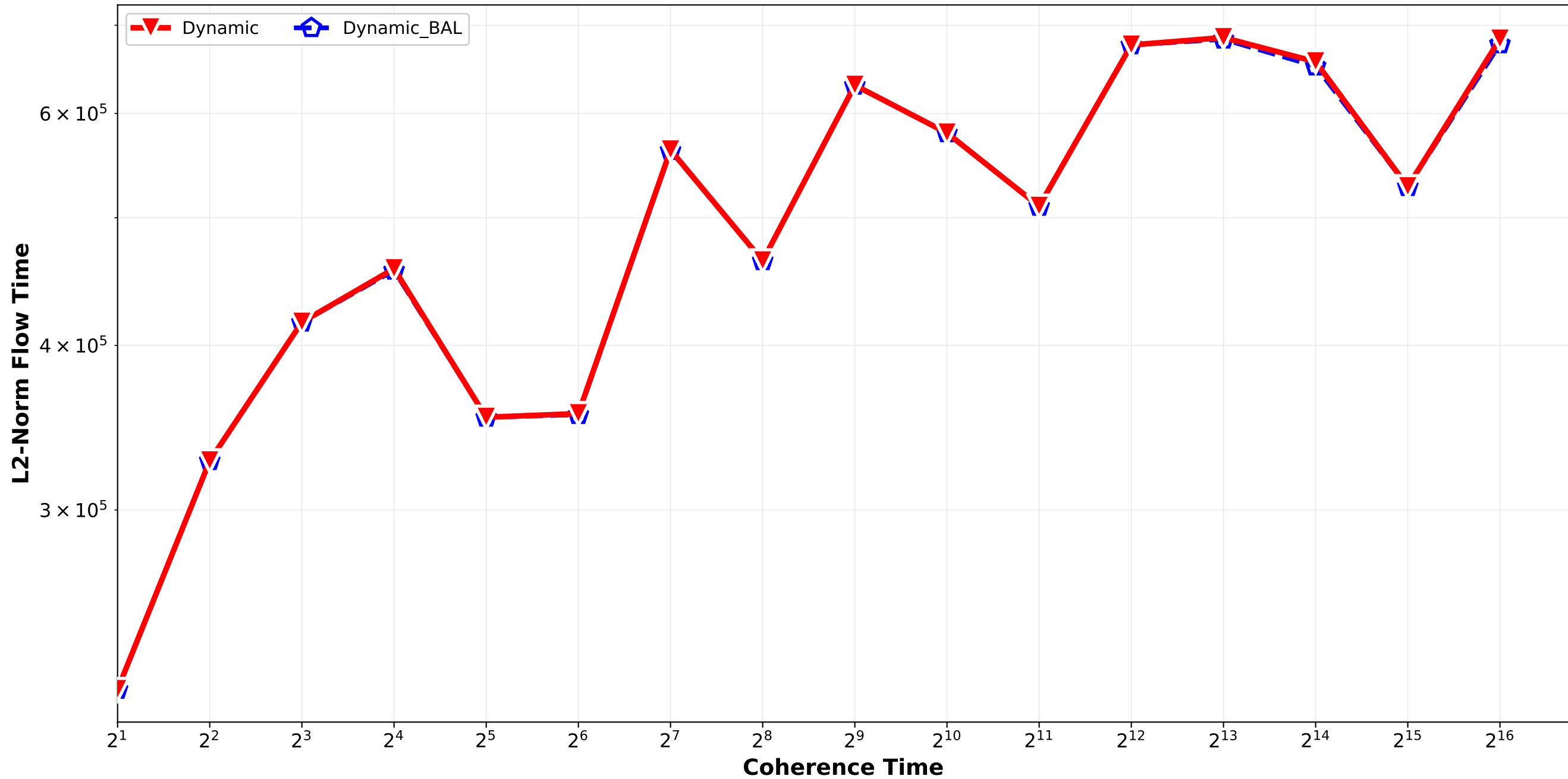
Dynamic vs Dynamic_BAL - L2 Norm Flow Time Bounded_Pareto_combination_softrandom H512_H4096 / pair_2
