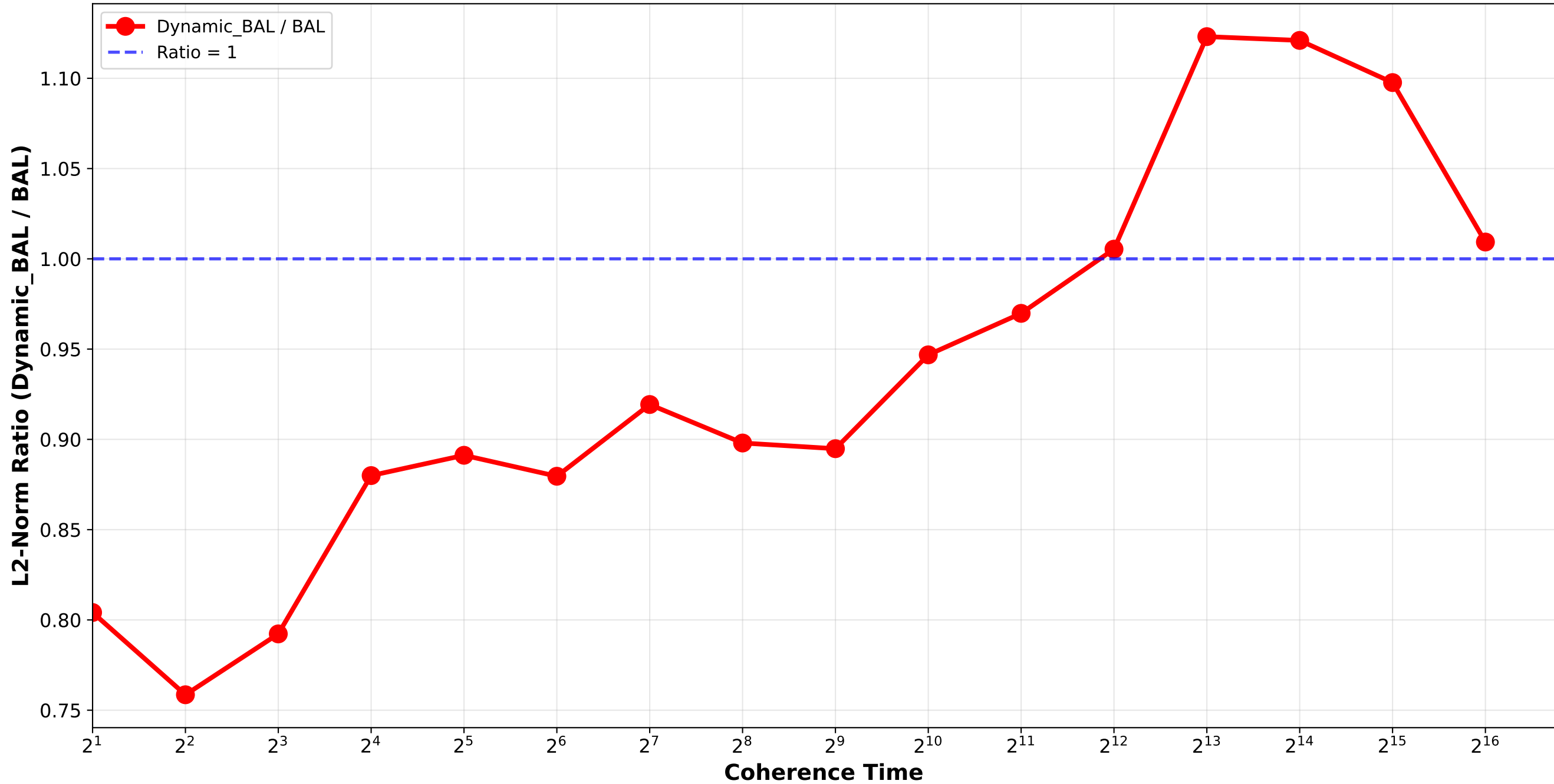
Dynamic_BAL vs BAL - L2 Norm Ratio Bounded_Pareto_combination_softrandom H64_H512 / pair_1
