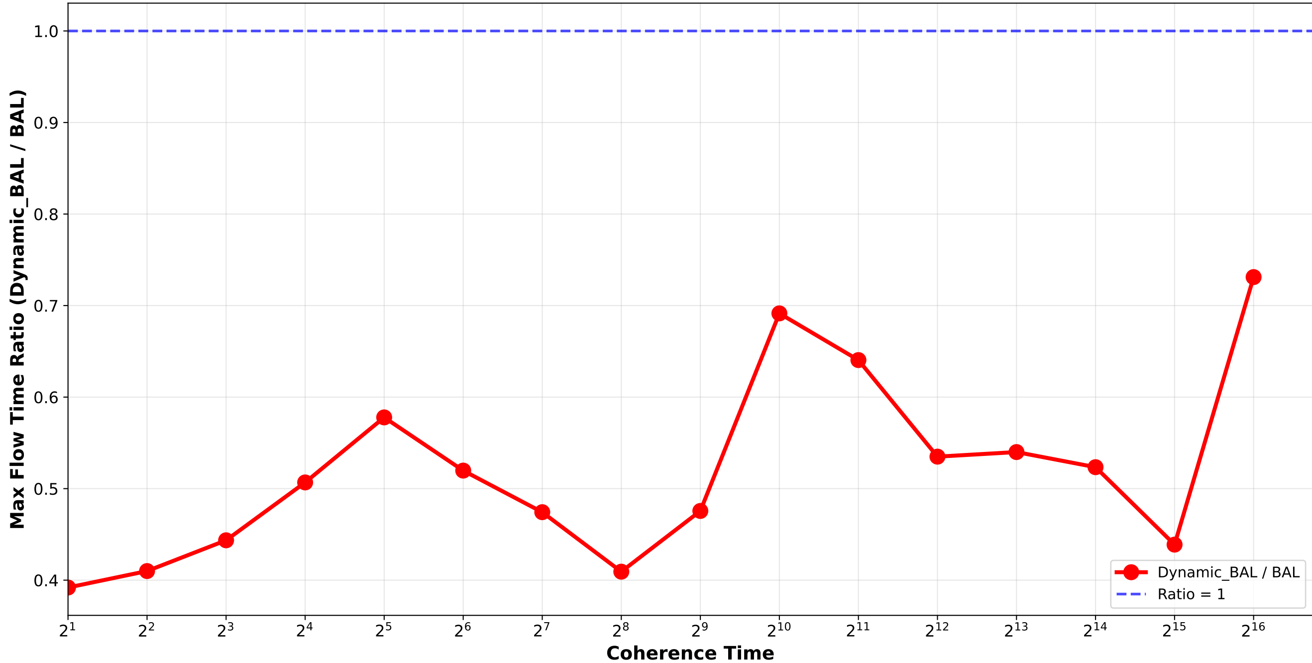
Dynamic_BAL vs BAL - Max Flow Time Ratio Bounded_Pareto_combination_softrandom H64_H512 / pair_1
