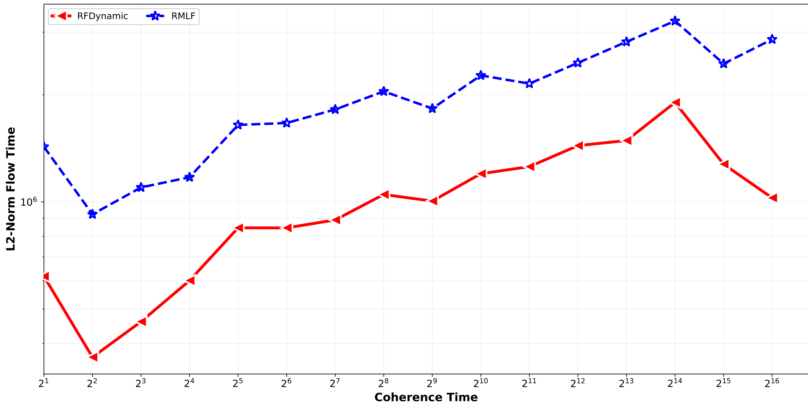
RFDynamic vs RMLF - L2 Norm Flow Time Bounded_Pareto_combination_softrandom H64_H512 / pair_1
