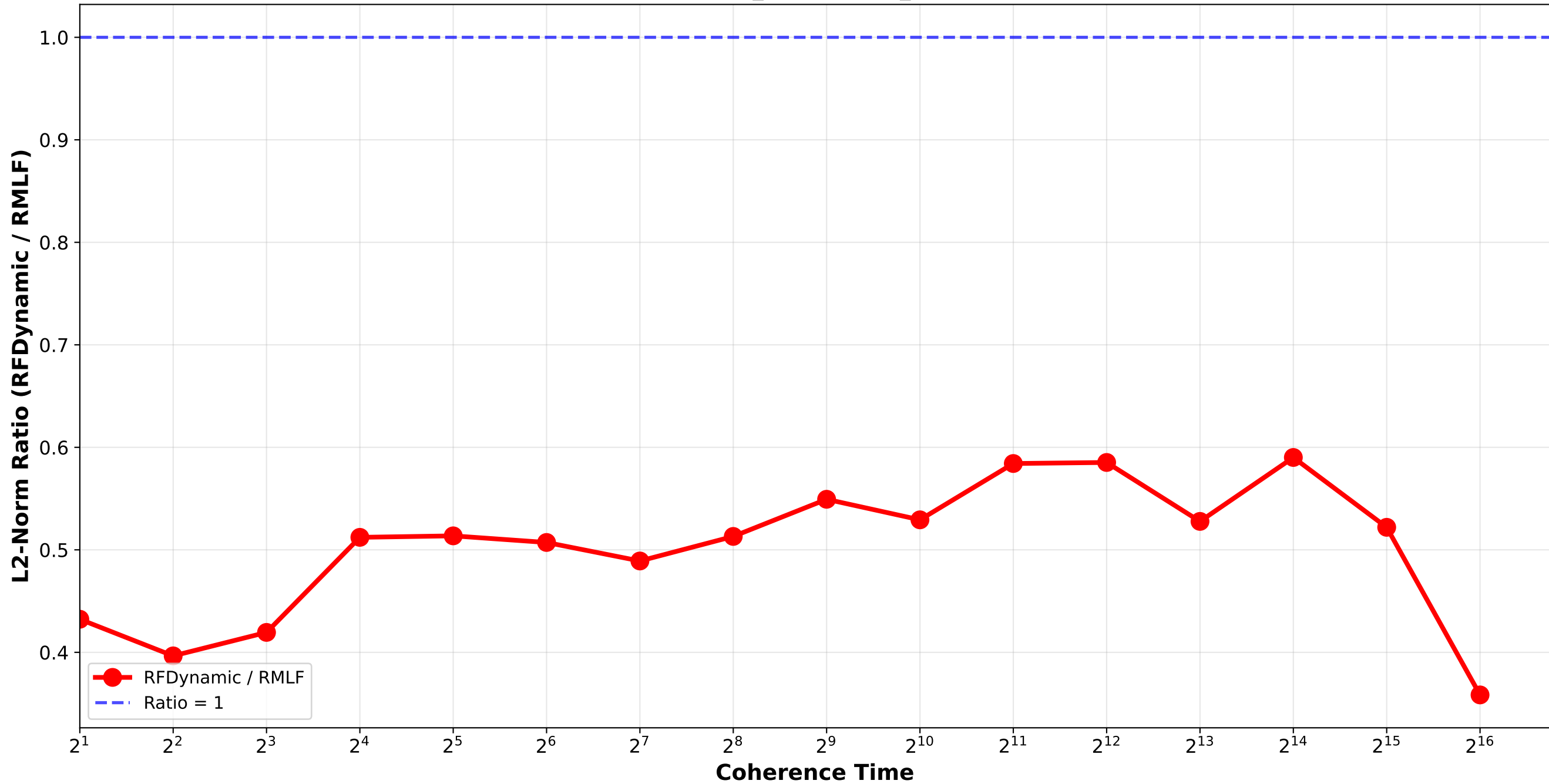
RFDynamic vs RMLF - L2 Norm Ratio Bounded_Pareto_combination_softrandom H64_H512 / pair_1
