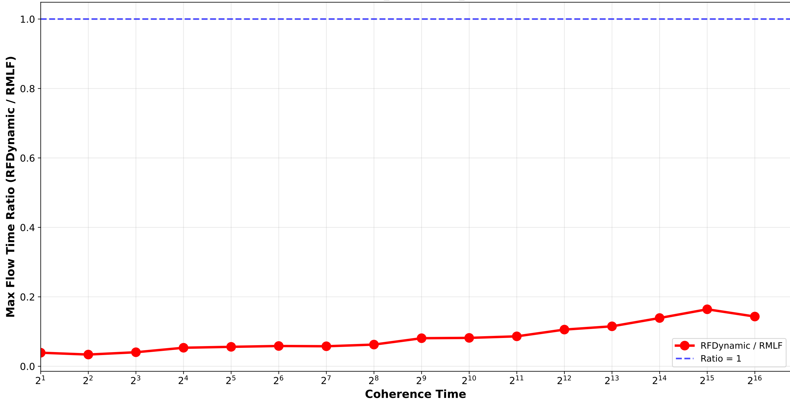
RFDynamic vs RMLF - Max Flow Time Ratio Bounded_Pareto_combination_softrandom H64_H512 / pair_1
