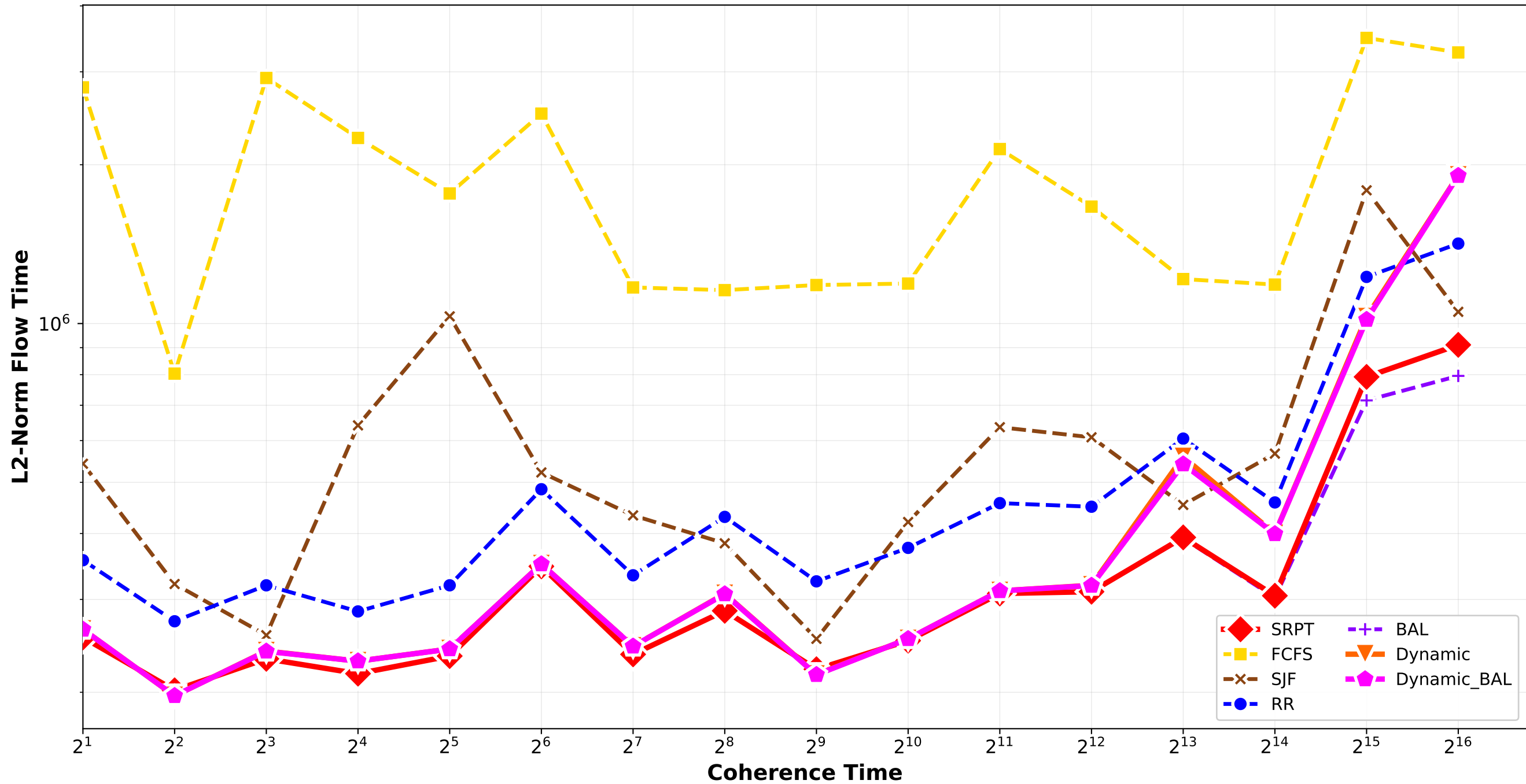
Clairvoyant Algorithms - L2 Norm Flow Time Bounded_Pareto_random
