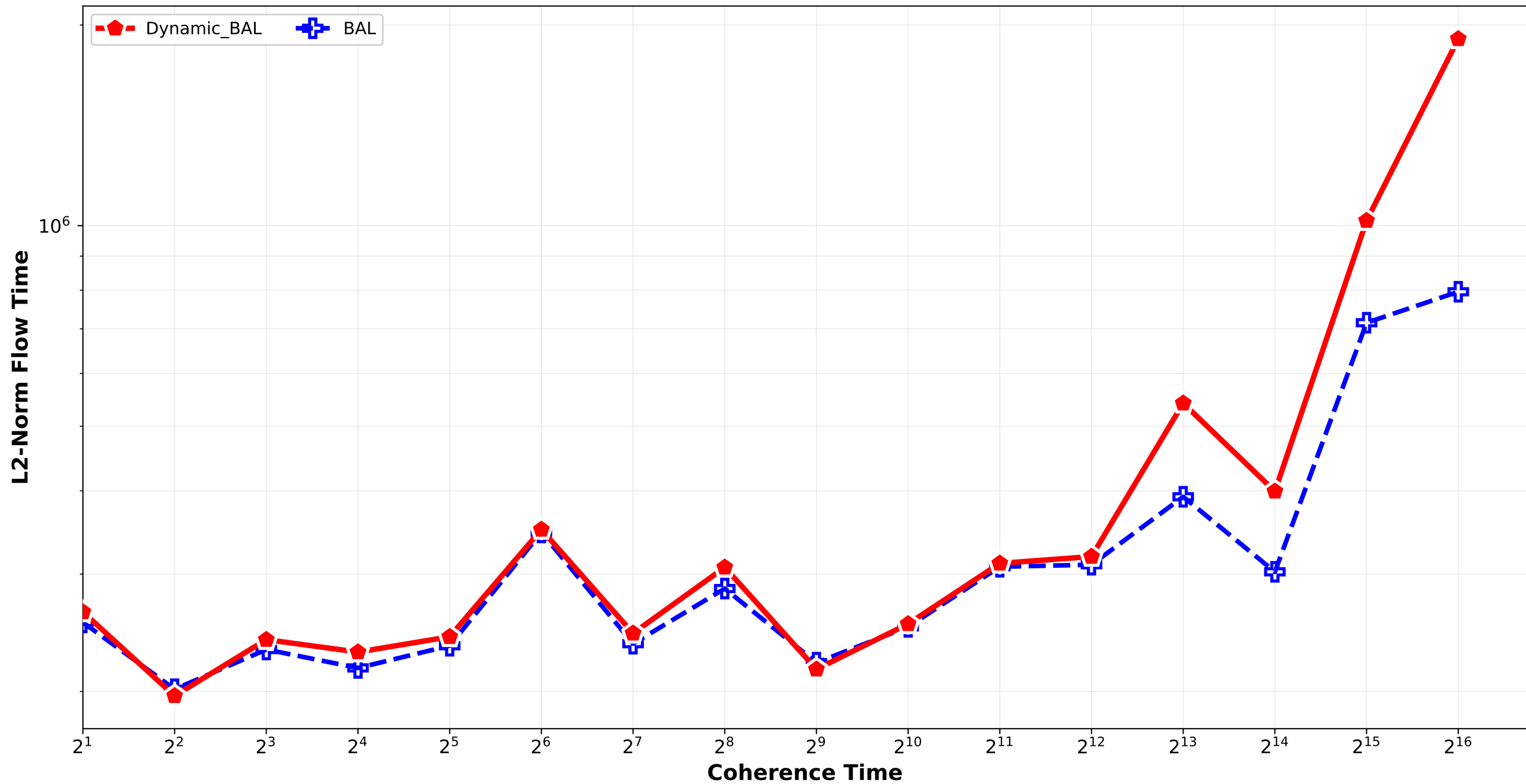
Dynamic_BAL vs BAL - L2 Norm Flow Time Bounded_Pareto_random
